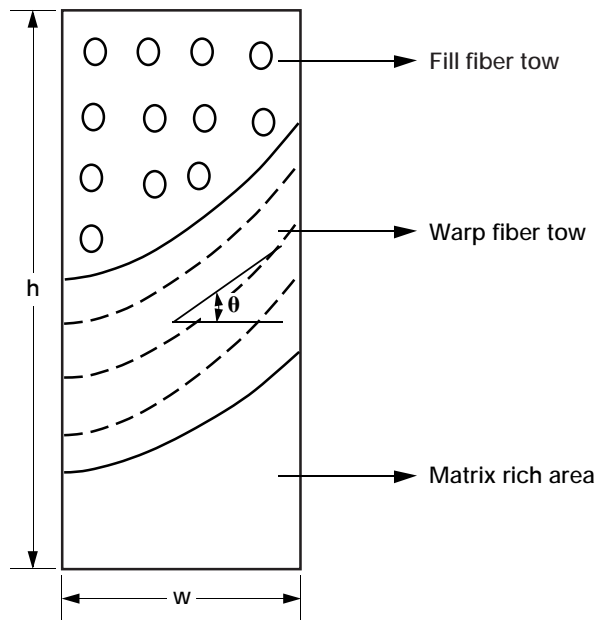
Figure 4.—A typical slice showing warp, fill and matrix regions.
