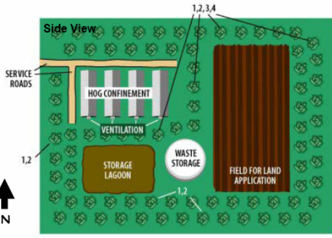
Figure 12. A hypothetical windbreak design for a swine facility. The numbers refer to the interaction and means by which the windbreak will mitigate livestock odor. 1. Creation of air mixing turbulence 2. Dust deposition 3. Particulate interception 4. Pollution sinks Other important design considerations include: livestock type, odor sources, air/wind patterns, tree/shrub species, and aesthetics.
