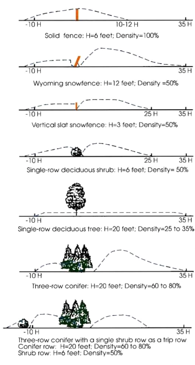
Figure: The height and density of the snow fence or windbreak will determine how much snow can be stored in the system.
