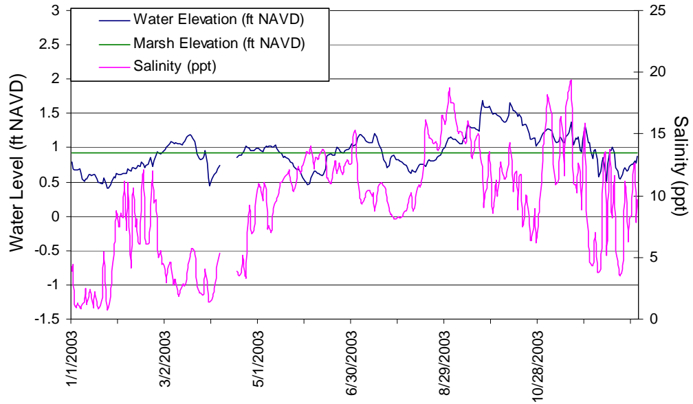
Figures 7. Hourly salinity and water level data at station CS17-02R in the borrow canal. Water level readings above marsh elevation indicate that the marsh was flooded.
