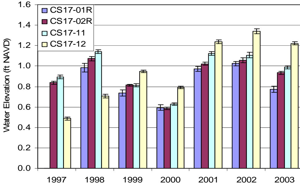
Figure 13. Yearly water levels at each of the stations since 1997. Station CS17-12 has increased relative to the reference stations since 1997.
