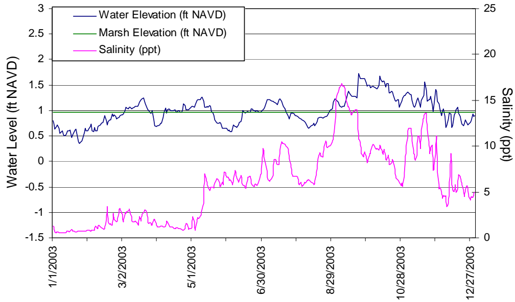
Figure 8. Hourly salinity and water level data at station CS17-11 in the northern project area. Water level readings above marsh elevation indicate that the marsh was flooded.
