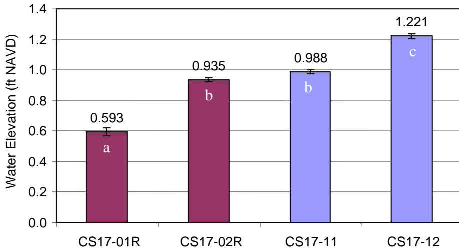
Figure 12. Yearly mean water level of daily means for 2003 at each CS-17 recorder (Mean \pm SE). Water elevation at CS17-01R, the recorder in the lake, was found to be significantly lower than at the other three recorders. CS17-12, the recorder in the southern project area, was found to be higher than the other recorders. Levels not connected by the same letter are significantly different.
