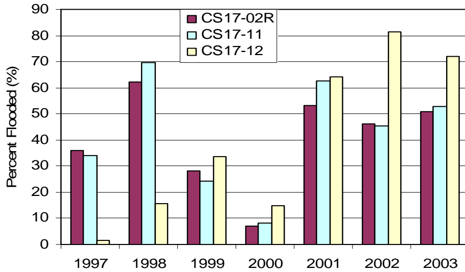
Figure 14. Percent of time the marsh was flooded at recorder stations in the CS-17 project area. Station CS17-12 has increased since 1999 relative to the reference recorder.
