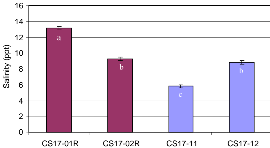
Figure 10. Yearly mean salinity of daily means for 2003 at each CS-17 recorder (Mean \pm SE). CS17-01R, the recorder in the lake, was found to be significantly higher than the other three recorders. CS17-02R, the recorder in the borrow canal, was found to be higher than CS17-11 (in the northern project area) but not CS17-12 (in the southern project area). Levels not connected by the same letter are significantly different.
