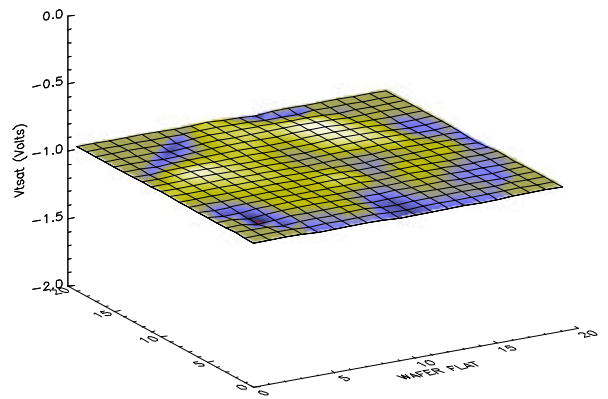
Figure 11. Threshold voltage for 2 \mu\text{m} channel length, p-channel transistors.
