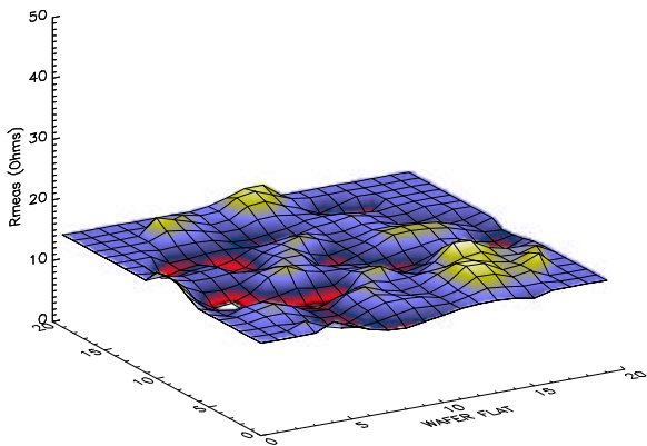
Figure 8. Source/drain contact resistance for 2 \mu\text{m} x 2 \mu\text{m} contacts to p-channel devices.
