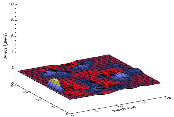
Figure 7. Source/drain contact resistance for 2 \mu\text{m} x 2 \mu\text{m} contacts to n-channel devices.
