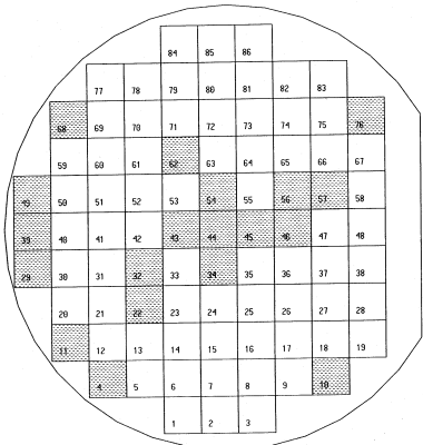
Figure 6. A wafer map from the first run showing functionality of wafer-level tests of combustible gas sensor devices. The unshaded devices are functional. The shaded devices are not functional.
