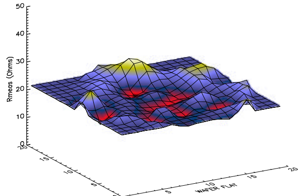
Figure 9. Metal to poly contact resistance.
