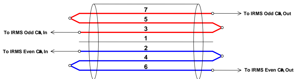
Figure 4.3: Illustration of the grouping of the conductors in a single 7-conductor cable with conductors 2, 4 & 6 connected to one IRMS channel and conductors 3, 5 & 7 connected to a second IRMS channel. This configuration was used when testing cable bundles in order to determine the relative timing of intra-cable faults, faults to an external ground, and inter-cable faults in support of efforts to resolve Bin 2 Items A and B.
