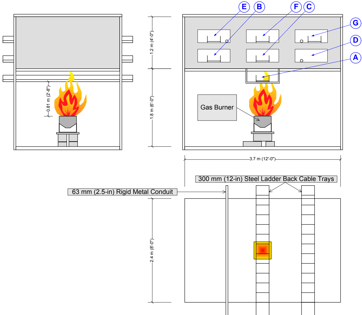
Figure 3.6: Schematic representation of the CAROLFIRE intermediate-scale test structure. Note the illustration of raceway locations A-G in the elevation view figure to the upper right. These are the same letter designations used in the test matrices (Section 5) to identify cable and raceway locations. The lower illustration is a plan view looking down onto the stacked raceways (one conduit and two stacks of cable trays are shown simply to illustrate the general placement).
