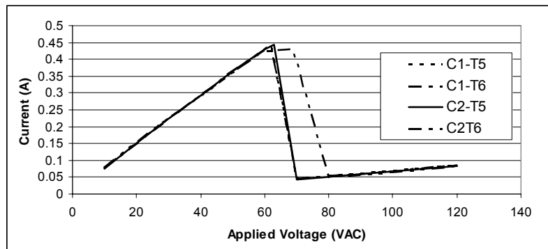
Figure C.9: Current draw of motor contactors versus applied voltage.
