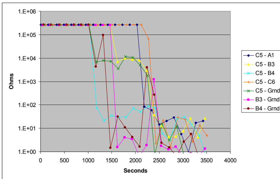
Figure 7.2: Illustration of the Inter-cable shorting behaviors observed by the IRMS in Test IT-1.
