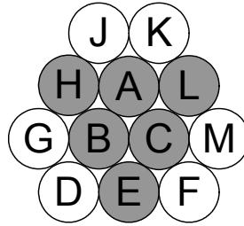
Figure 7.1: Illustration of the letter code used to identify cables when testing 12-cable bundles. Only the shaded cables are monitored for electrical performance. The corresponding letter codes for testing of three- and six-cable bundles are presented in Figure 6.1 above.
