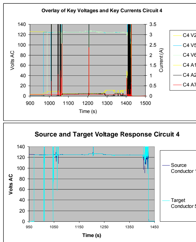
Figure 7.4: Results for SCDU-4 in Test IT-9.
