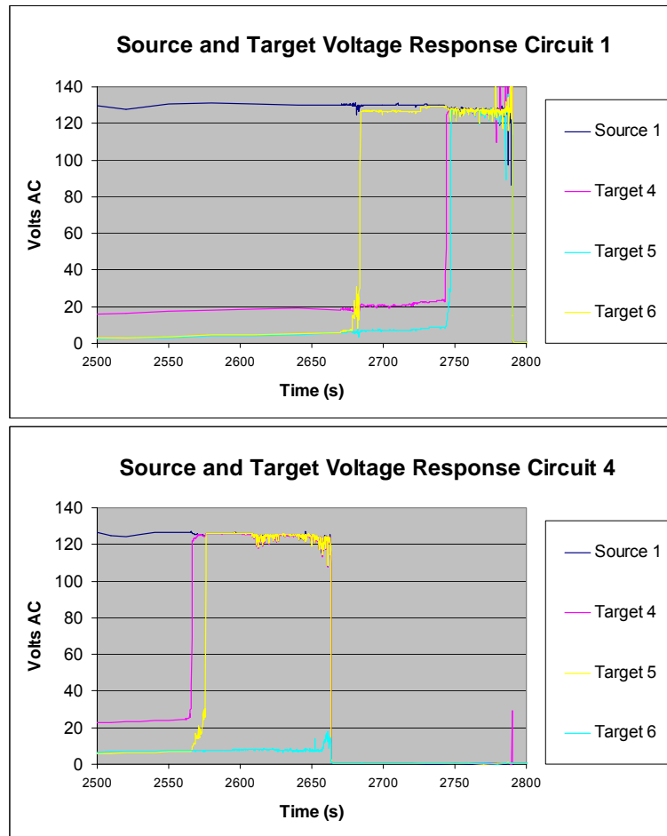
Figure 7.6: Illustration of the inter-cable interactions observed between circuits 1 and 4 in Test IT-1. Note the voltage spike to Target 4 in Circuit 4 after that circuit had experienced a fuse blow.
