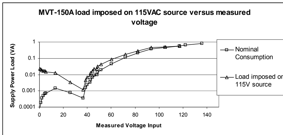
Figure D.12: Power consumption imposed on the CPT by the NEI/EPRI style voltage transducers.
