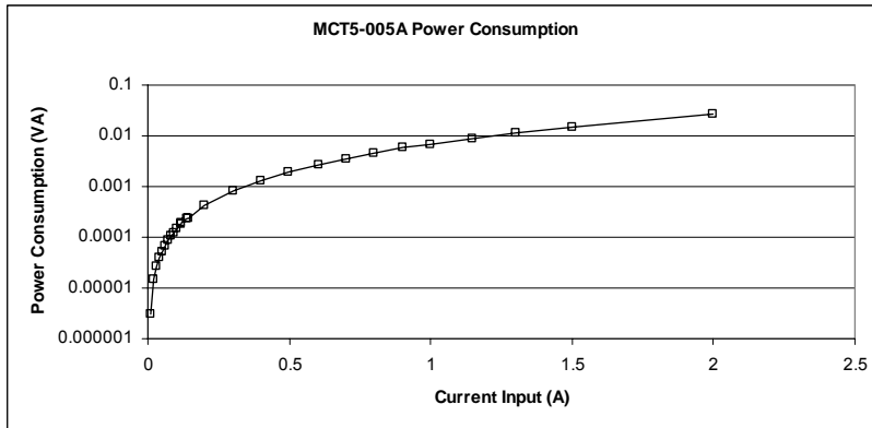
Figure D.10: Power consumption behavior for the NEI/EPRI style current transducers.
