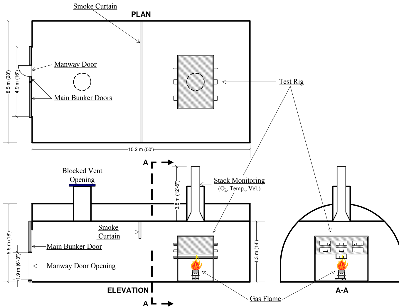
Figure 3.7: Schematic representation of the CAROLFIRE intermediate test structure located within the outer test facility.
