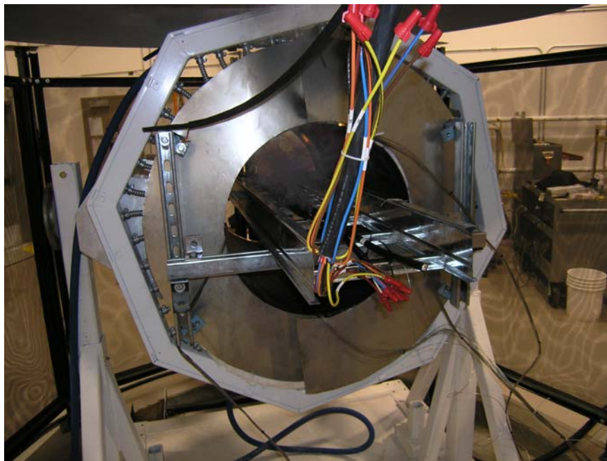
Figure 3.1: General view of the Penlight Facility with the cable tray in place and a test in progress. Note that this view shows Penlight in an ‘open-ends’ configuration used in many of the Penlight Preliminary Tests.
