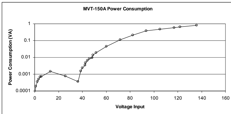
Figure D.11: Power consumption behavior for the NEI/EPRI style voltage transducers.
