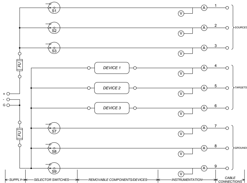
Figure C.8: Generic design of the SCDUs.
