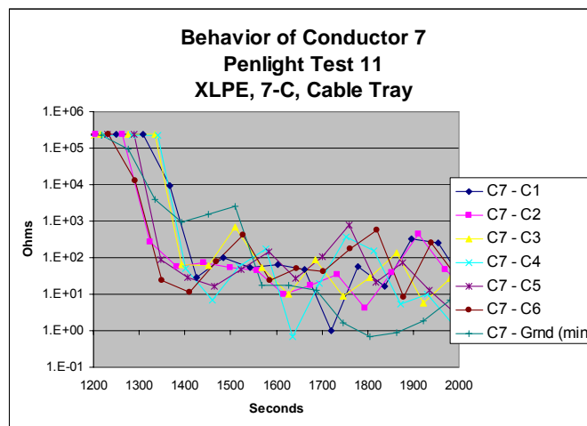
Figure 4.1: Example of a typical IRMS data plot taken from Penlight Test 11.
