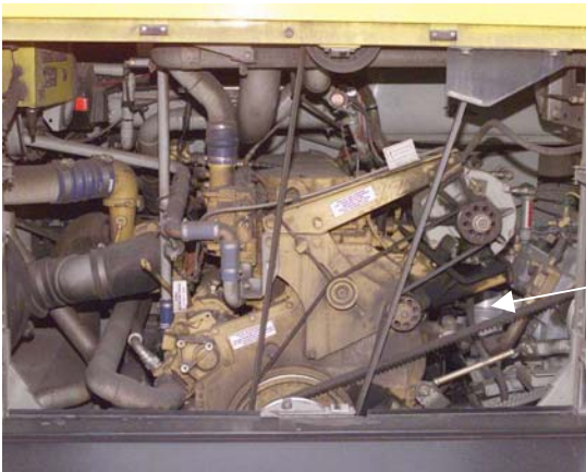
Figure 5. Close-up photograph of the Caterpillar engine compartment.
