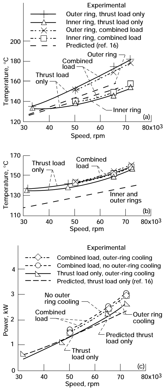
Figure 10.—Effect of speed on bearing temperature and power loss of split-inner-ring, 35-mm-bore, angular-contact ball bearing (design 1, fig. 2 (a)). Thrust load, 667 N (150 lbf); radial load, 222 N (50 lbf); nominal contact angle, 24°; cage, inner-ring, land-guided; type of lubrication, flow through split inner ring. (a) Ring temperature with no outer-ring cooling. (b) Ring temperature with outer-ring cooling. (c) Power loss.
