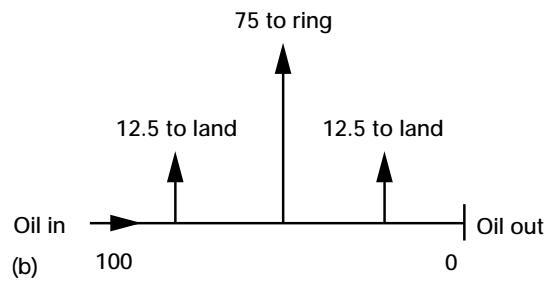
Figure 4.—Oil-flow distribution through inner ring. (a) 50 percent flow. (b) 75 percent flow.
