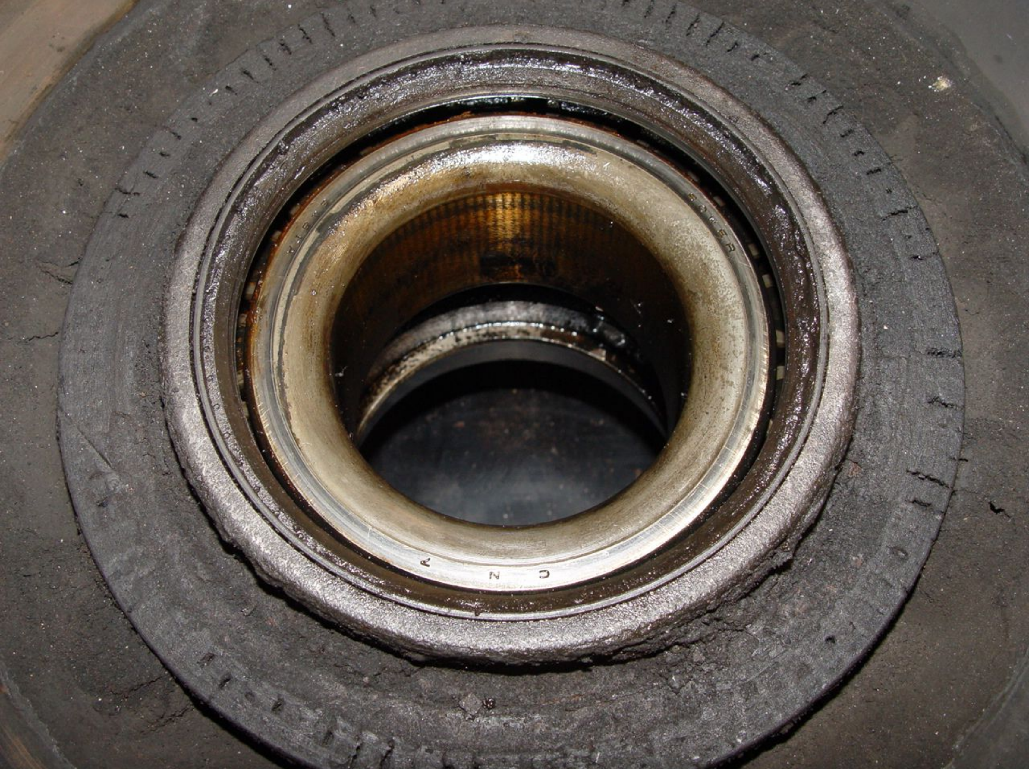
VEH Photo #24 - Left Side Tag-Axle Tone Ring With Oil (Source: Dallas County Sheriff's Dept.)
