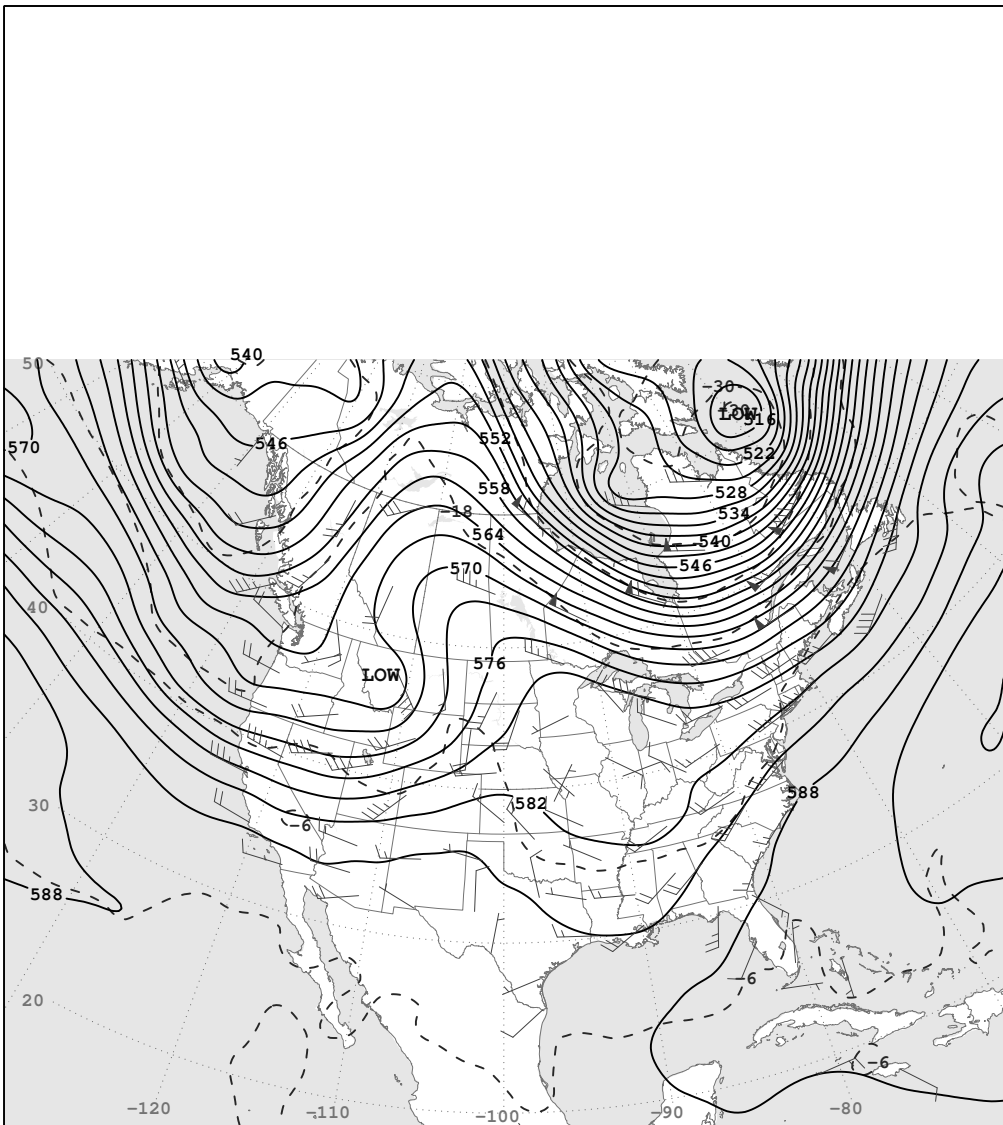
SUN, SEP 21, 2008 500-Millibar Height Contours at 7:00 A.M. E.S.T.
