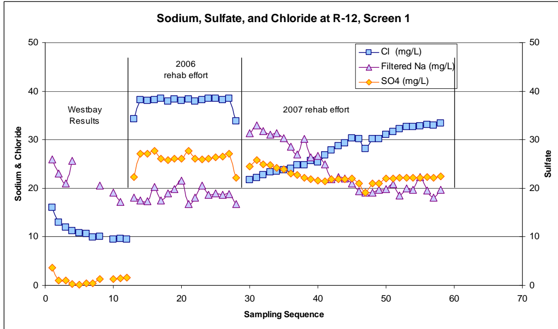
Figure 2.7-4 Sample sequence versus dissolved concentrations of sodium (Na), chloride (Cl), and sulfate (SO 4 ) during characterization sampling using Westbay equipment and pumping tests conducted in September 2006 and October 2007 at R-12 screen 1
