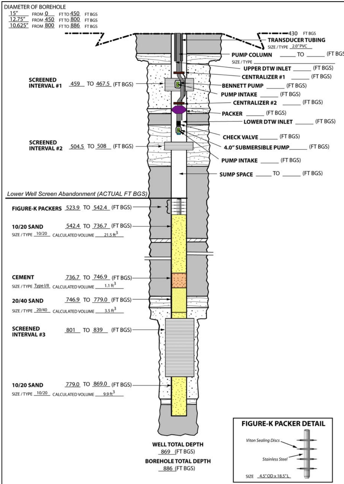
Figure 2.4-1 Abandonment and rehabilitation specifications regional well R-12
