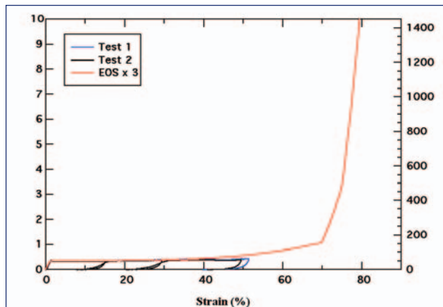
Figure 7. Stress-strain curve for thermal tile: blue and black are data, red is model.
