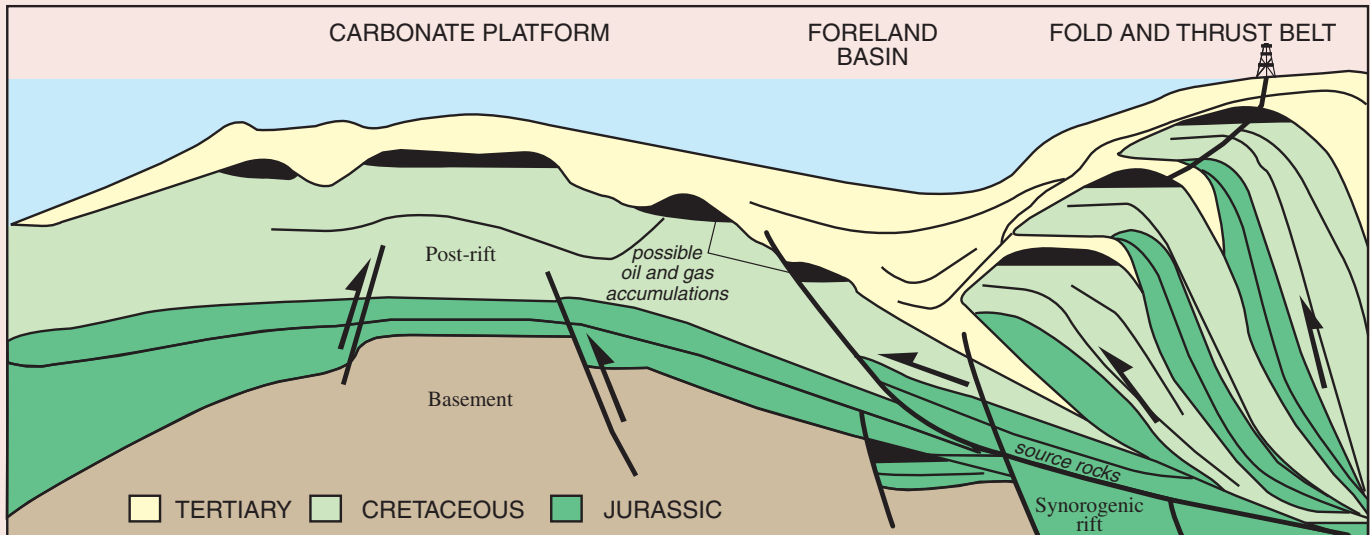
Figure 2. Schematic northwest–southeast cross section in the North Cuba Basin showing possible migration pathways of petroleum from source rocks within the fold and thrust belt into structures and reservoirs in the fold and thrust belt, in the foreland, and in the carbonate platform (after Magnier and others, 2004).
