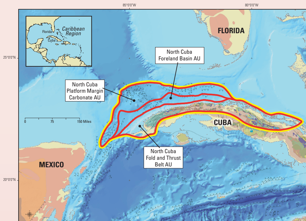
Figure 1. North Cuba Basin of northwestern Cuba. The Jurassic–Cretaceous Composite Total Petroleum System boundary (yellow line) encompasses the three assessment units (AU) defined and assessed in this study. Fine black lines on the ocean floor are faults; ball and bar on downthrown side.
