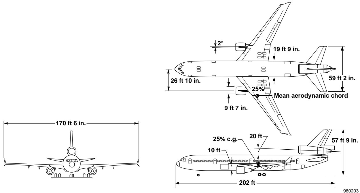
Figure 1. The MD-11 airplane.
