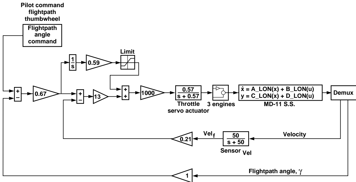
Figure 5. The MD-11 PCA longitudinal block diagram (autothrottle control) mode D.
