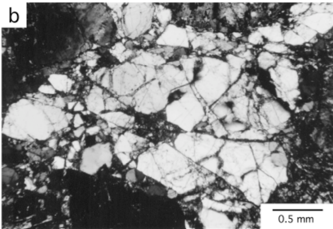
Figure 1. Photomicrographs of deformation and mineralization textures in core samples from the Nojima fault zone. a) The highest permeability measured by Naka et al. (1998) was in this NIED sample, 80-29, which contains a set of elongate dilational cracks that are lined but not filled with laumontite and carbonate minerals (crossed polarizers). b) Heavily fractured quartz in high-permeability NIED sample 43-37-1.
