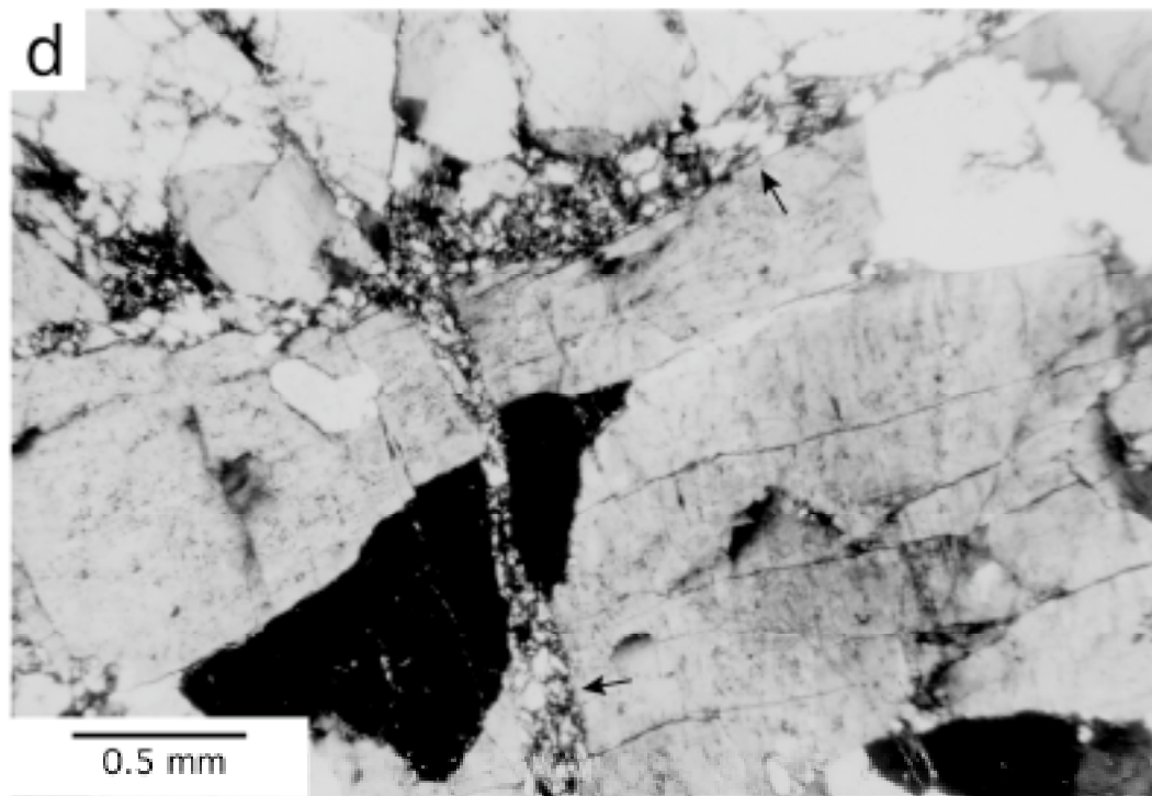
Figure 1, continued. c) Granulation of the igneous minerals leads to formation of fine-grained gouge of low strength and moderately low permeability. This gouge is cut by a dilational crack (indicated by arrows), filled with laumontite. The dark vertical lines contain carbonate minerals (GSJ 98-31, plane polarized light). d) Narrow microshears (indicated by arrows) parallel to the two prominent fracture orientations visible in the K-feldspar crystal at right (NIED 183-14C, crossed polarizers).
