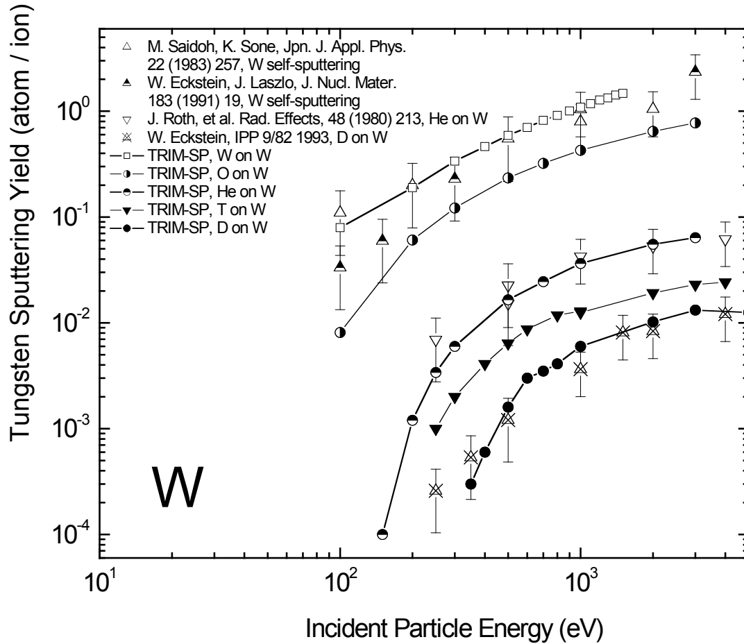
FIG. 3 Tungsten sputtering yield computational simulations with TRIM-SP compared to data. The yield is plotted against incident particle energy of D, T, He, O and W. The light particles are simulated at 45-degrees incidence and W at 30-degrees incidence with respect to the sample surface normal.
