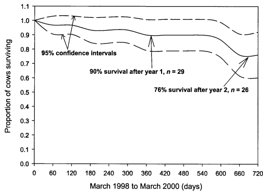
Fig. 2. Survival estimates for cow moose in eastern interior Alaska, USA, 1998–2000, using Kaplan-Meier method with staggered entry design.
