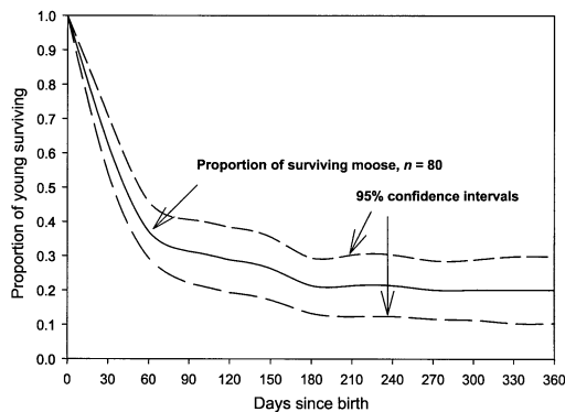
Fig. 3. Survival estimates for calf moose in eastern interior Alaska, USA, 1998–2000, using Kaplan-Meier method with staggered entry design.
