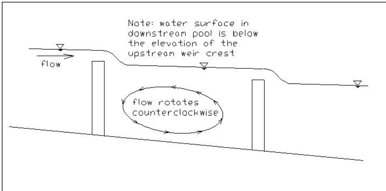
Figure 1-1. Plunging Flow over Fishway Weir
