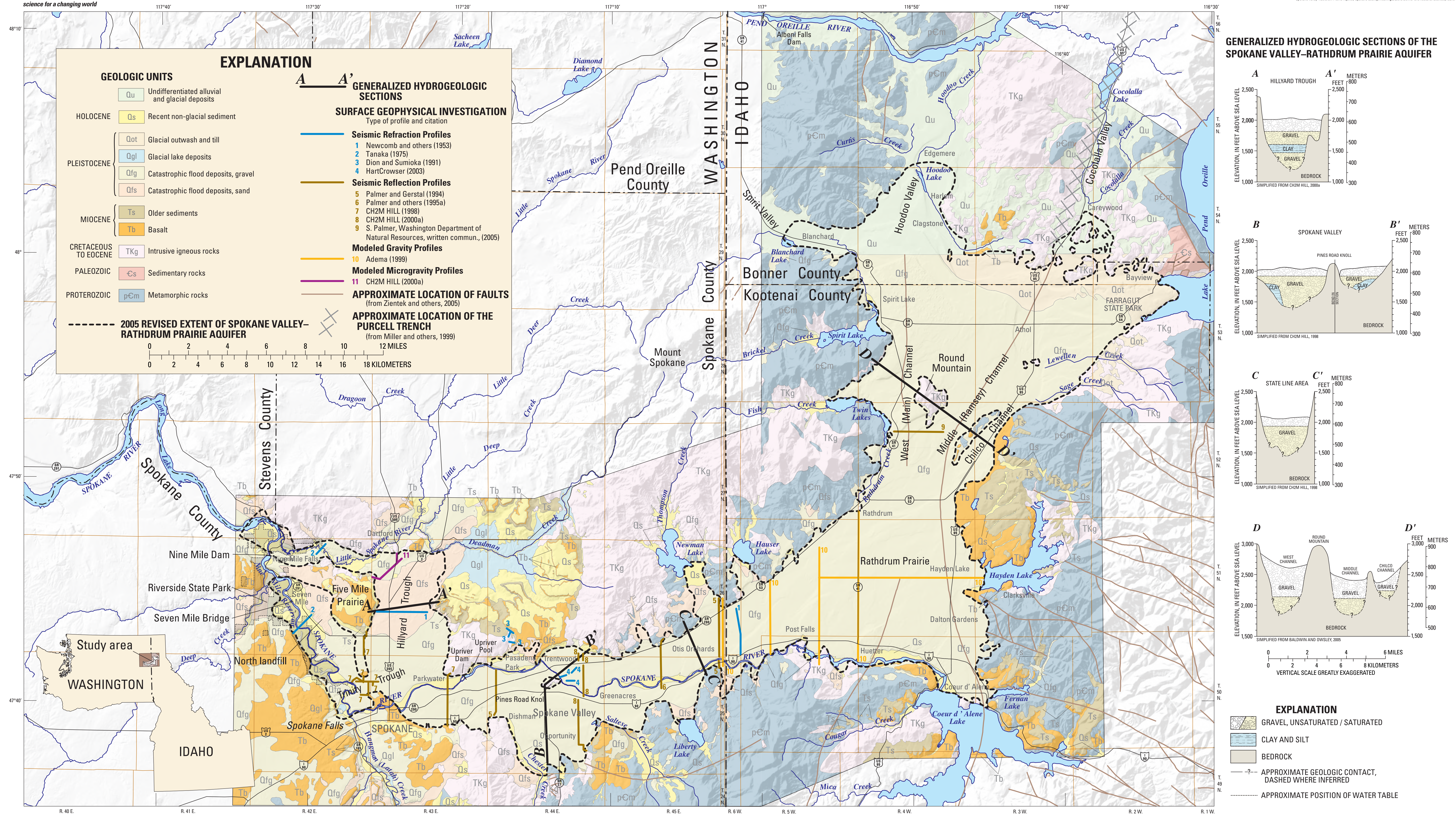
SIMPLIFIED SURFICIAL GEOLOGY, GENERALIZED HYDROGEOLOGIC SECTIONS, AND SURFACE GEOPHYSICAL TRANSECTS, SPOKANE VALLEY-RATHDRUM PRAIRIE AQUIFER, WASHINGTON AND IDAHO
