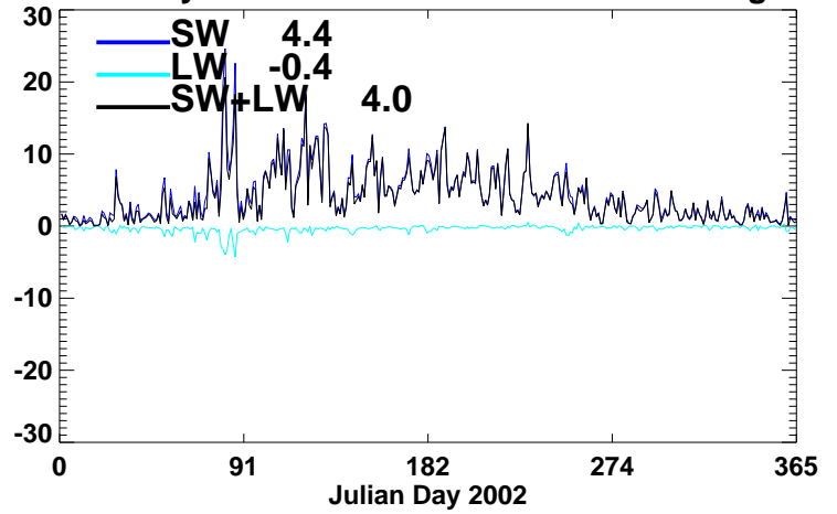
All Sky SURFACE Net Aerosol Forcing
