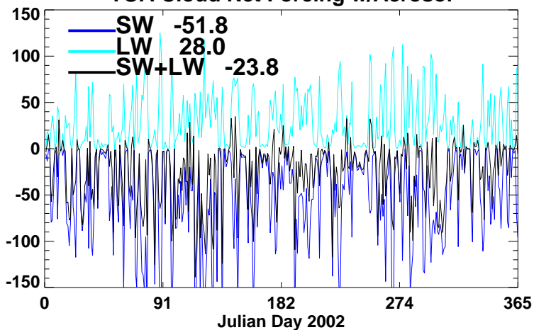
ATM Cloud Net Forcing w/Aerosol
