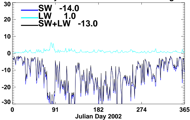
Clear Sky SURFACE Net Aerosol Forcing
