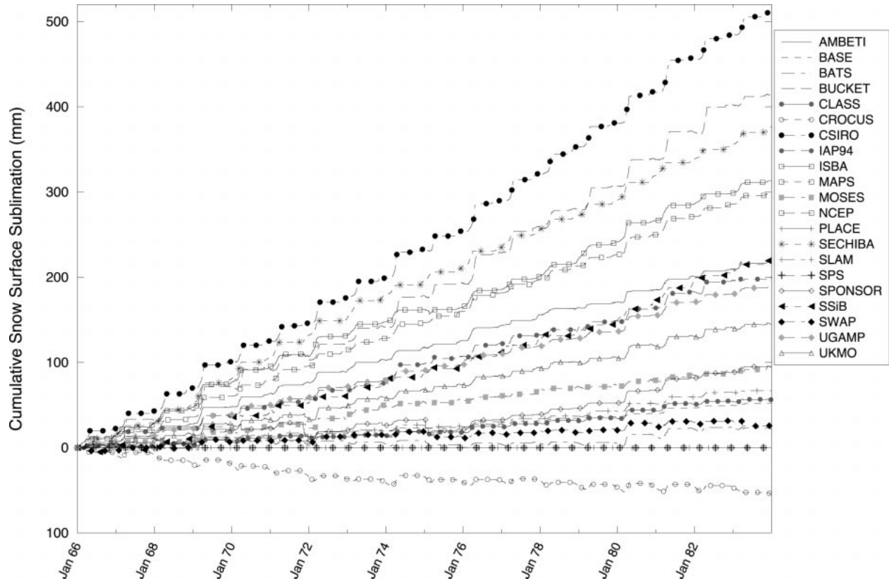
FIG. 2. The cumulative evaporation (mm) from snow over the 18 yr of the CTRL simulation. (PLACE did not report this variable.)
