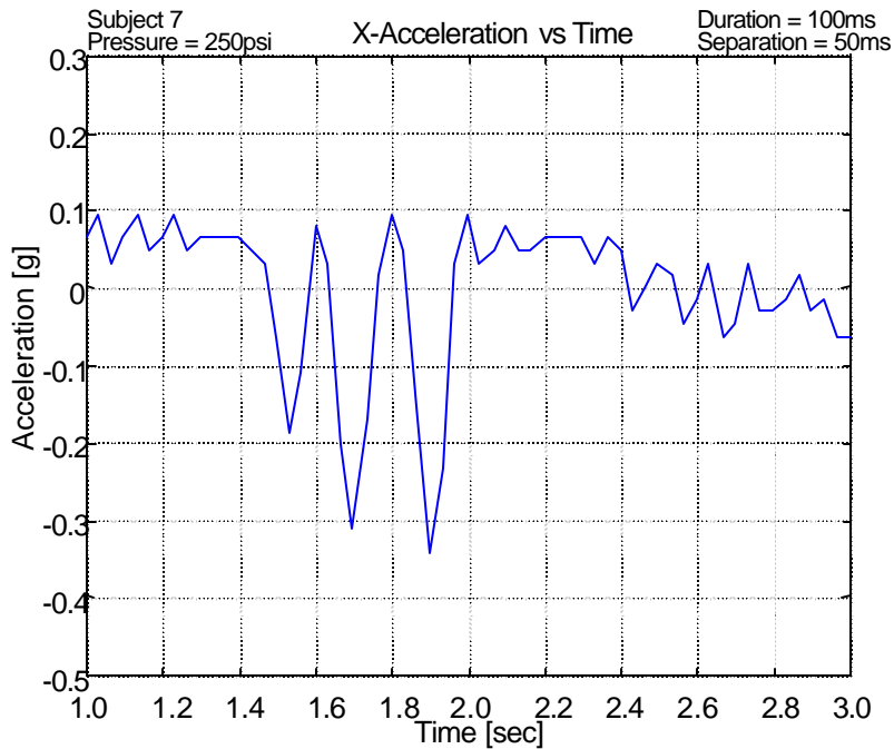
Figure 5-29 Acceleration Profile for Haptic Brake Pulses (100ms duration-50ms separation) at 250 psi
