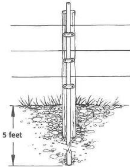
Fig. 3. Grounding rod for wire fences.
