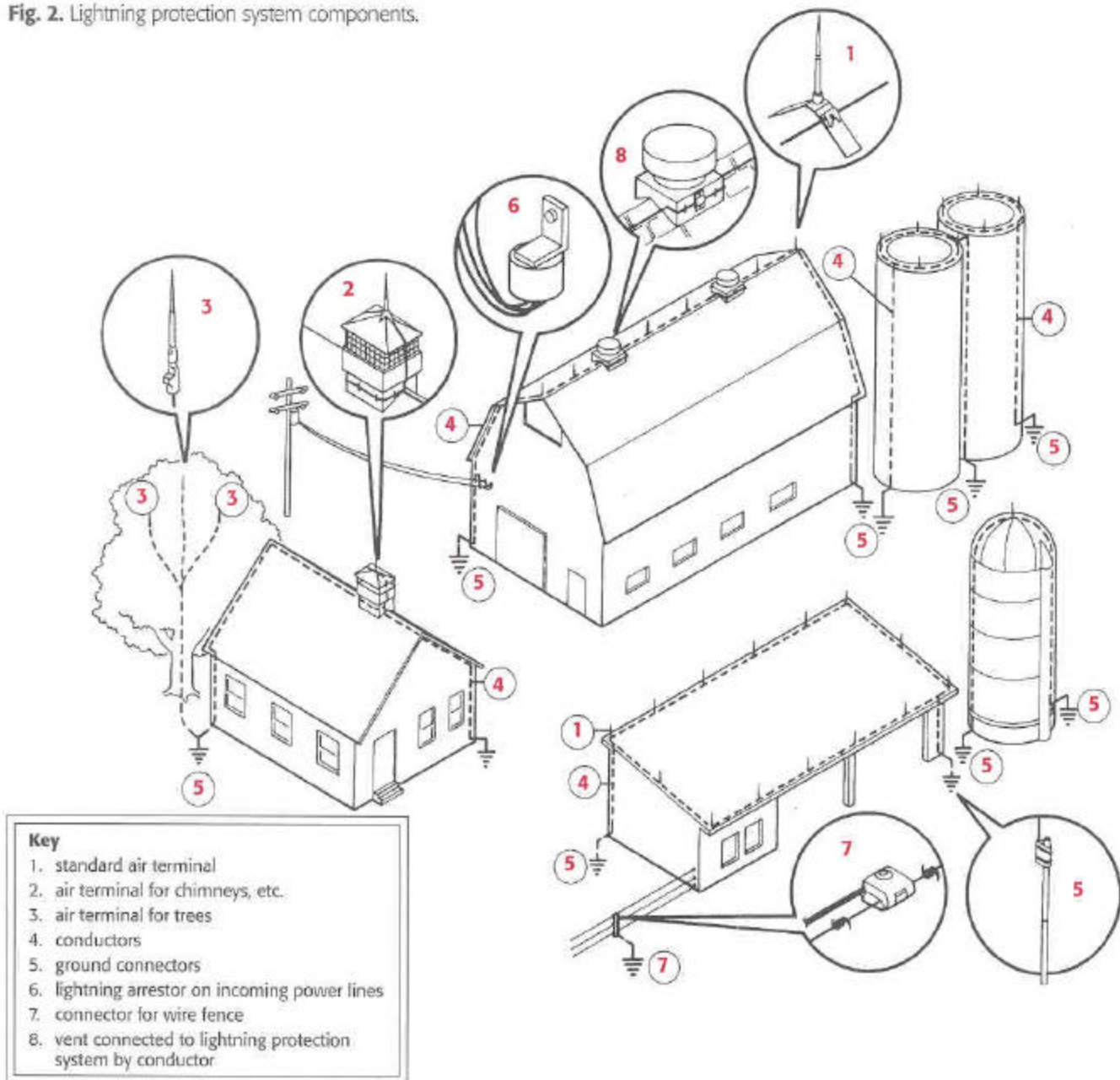
Fig. 2. Lightning protection system components.
