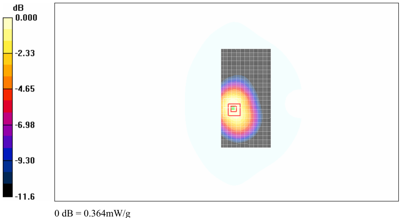
Fig. 29 CDMA 835MHz, Body, Towards Ground, CH1013
