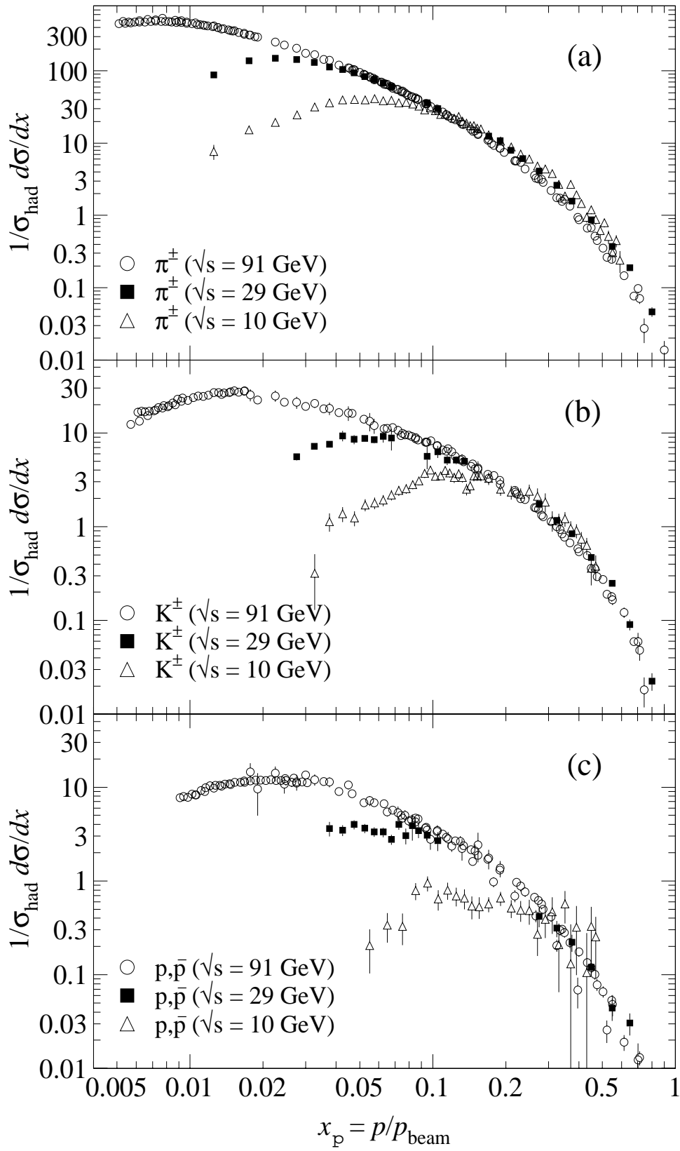
Figure 17.4: Scaled momentum spectra of (a) \pi^\pm , (b) K^\pm , and (c) p/\bar{p} at \sqrt{s} = 10 , 29, and 91 GeV are shown [7,23].
