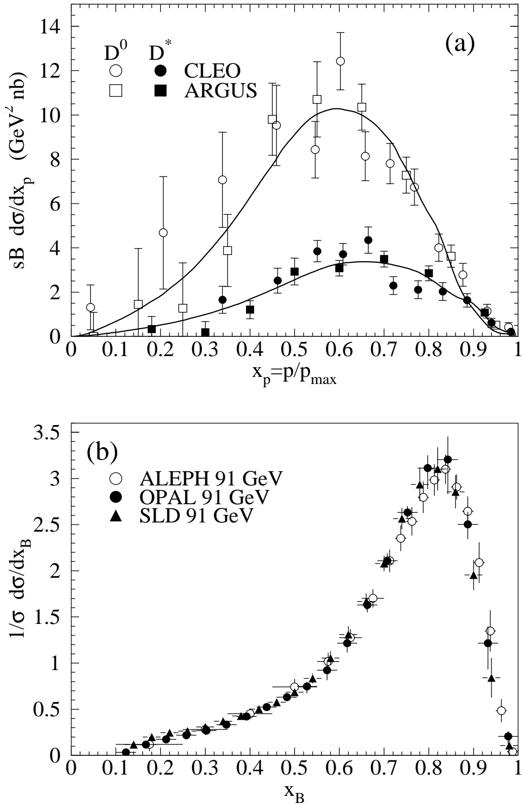
Figure 17.5: (a) Efficiency-corrected inclusive cross-section measurements for the production of D^0 and D^{*+} in e^+e^- measurements at \sqrt{s} \approx 10 GeV [35,40]. (b) Measured e^+e^- fragmentation function of b quarks into B hadrons at \sqrt{s} \approx 91 GeV [41,42].
