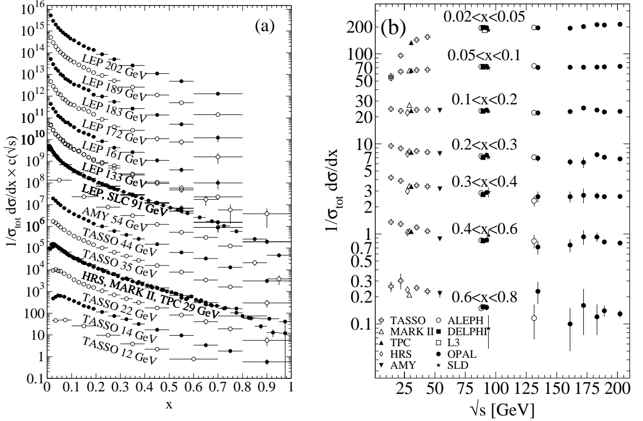
Figure 17.1: The e^+e^- fragmentation function for all charged particles is shown [6,7,8,9](a) for different c.m. energies, \sqrt{s} , versus x and (b) for various ranges of x versus \sqrt{s} . For the purpose of plotting (a), the distributions were scaled by c(\sqrt{s}) = 10^i where i is ranging from i = 0 ( \sqrt{s} = 12 GeV) to i = 13 ( \sqrt{s} = 202 GeV).
