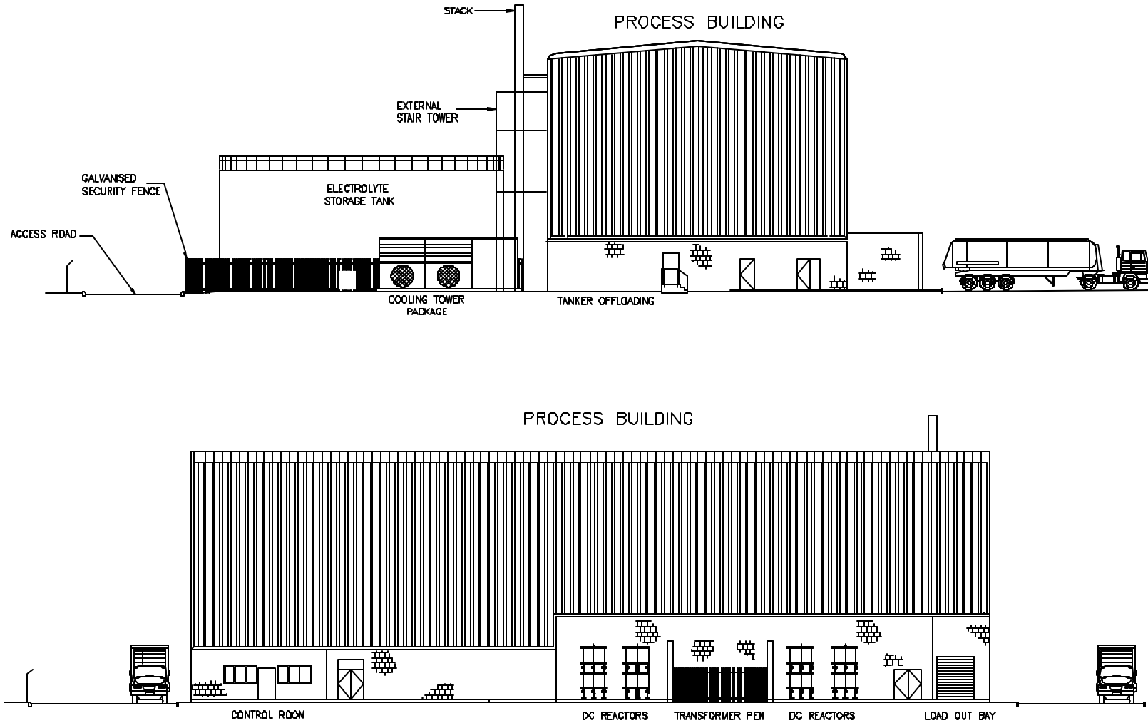
Figure B-4 Regenesys™ Elevation View
