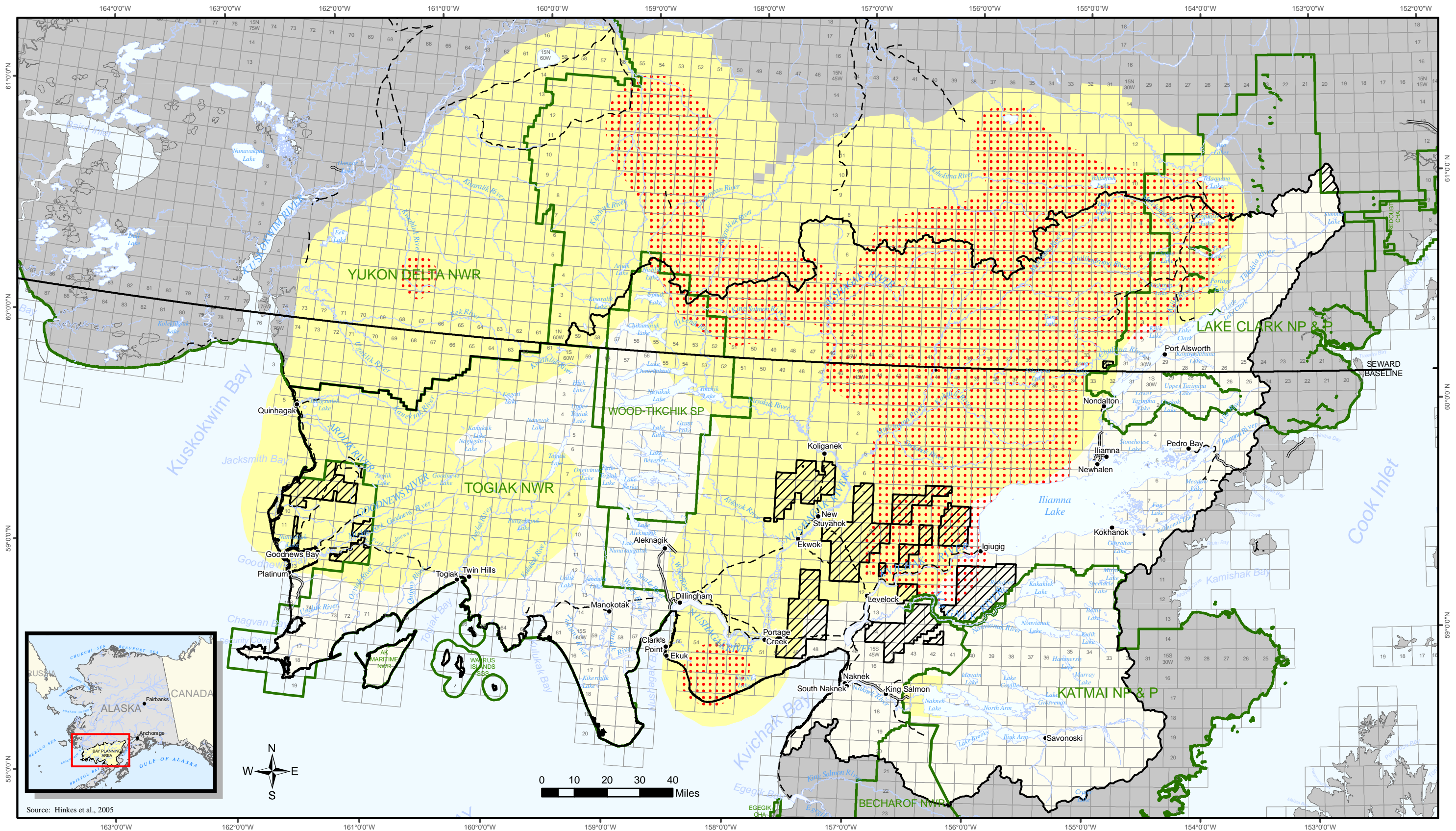
Range (95% fixed kernel) of the Mulchatna Caribou Herd before/after the 1994 shift to the west, southwest Alaska Map 3.15
