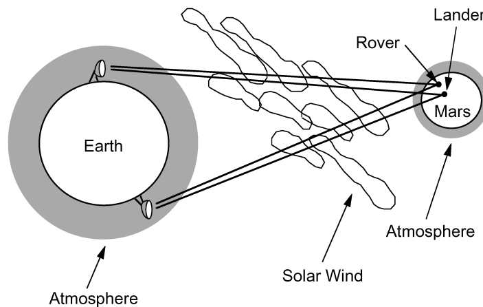
Fig. 5-1. Same-beam interferometry measurement geometry.
