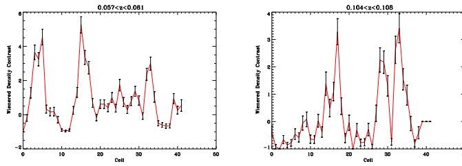
Figure 3. The plot of overdensities in SGP for the each redshift slice for 10h^{-1} Mpc target cell size shown above. Also plotted are the variances of the residual associated for each cell. The increase in cell number indicates the increase RA in each redshift slice.
