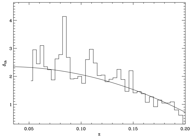
Figure 6. The density threshold \delta_{th} as a function of redshift z and the best fit model used to select the superclusters in Table 1.
