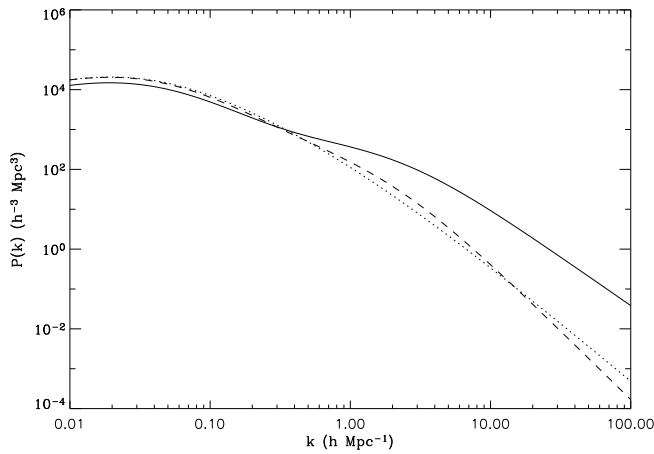
Figure 5. Non-linear power spectra for z=0 and the concordance model with \sigma_p = 506 \text{ km s}^{-1} in real space (solid line), in redshift space from equation 42 (dashed line), both derived using the fitting formulae of Smith et al. (2003) and linear power spectra in redshift space derived using linear theory and Kaiser’s factor (dotted line).
