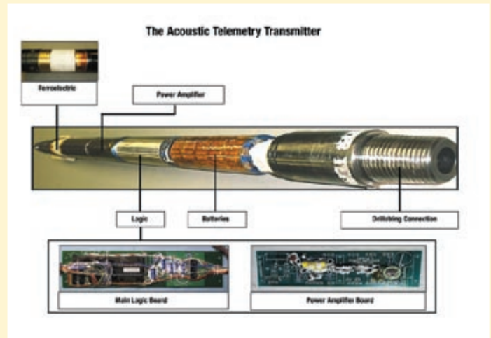
Acoustic telemetry device quickly and reliably transmits data to the surface of a geothermal well to improve drilling, increase production, and lower well costs.
