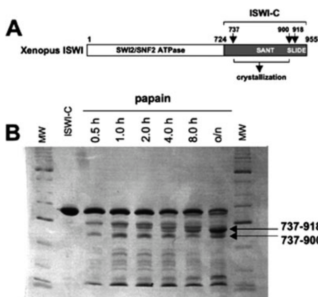
Fig. 1. (A) Schematic representation of Xenopus ISWI. Arrows and residue numbers label proteolytic cleavage sites. (B) A recombinant fragment of Xenopus ISWI-C (amino acids 724–955) was subjected to partial proteolysis using papain protease for various times. The products were resolved by SDS-PAGE.
