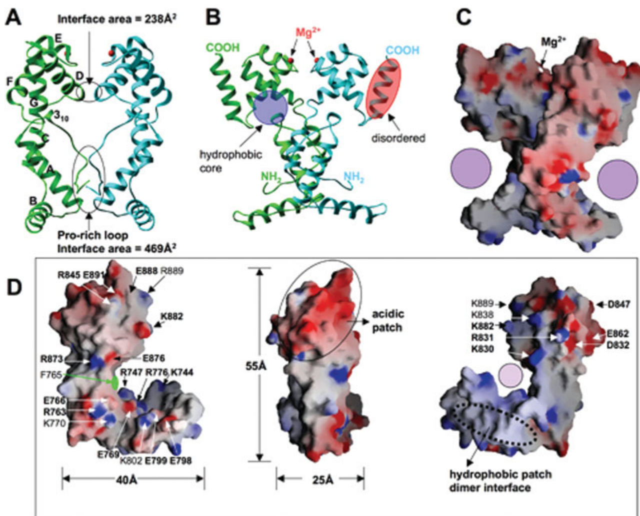
Fig. 2. Structure of Xenopus SANT. (A) A dimer of SANT domain formed in the crystallographic asymmetric unit. The dimer interface is formed between the N-terminal Pro-rich loop—hydrophobic interactions involving proline residues (P743, P746, P748, and P749) and helix \alpha A (Tyr775 and Tyr781) - and the helix \alpha D (two salt bridges between invariant Arg803 of one protomer and invariant Asp804 of another protomer). The Stokes radius of the domain was consistent with a solution dimer: the 21-kDa protein eluted from S75 gel filtration column with apparent molecular weight of 41 kDa. The total area of dimer interface of 707 Å 2 is within the limits, though at the lower end, of the 32 homodimers examined. 9 (B) A 90° rotated view from panel A. A Mg 2+ ion, required for crystallization, is bound at the loop region between helices \alpha E and \alpha F. Three main chain carbonyl oxygen atoms of Ala852, Val855, and Lys858 and two water molecules (w) coordinate the metal atom. (C) GRASP surface charge distribution is displayed with blue for positive, red for negative, and white for neutral. Filled circle indicates the opening of the concave L-surface. (D) Three views of the monomer structure of Xenopus SANT domain.
