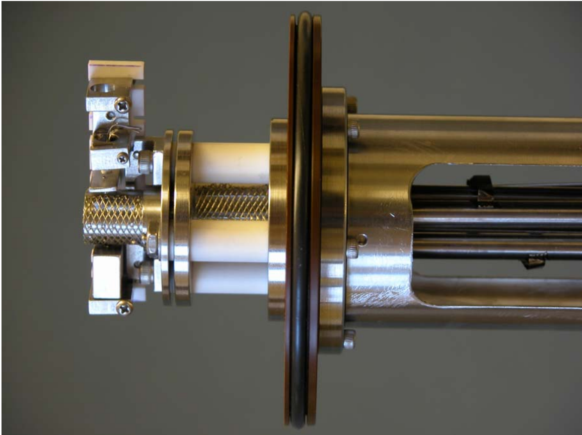
Fig.2. Photograph of the ionizer and ion optics mounted on the QMS. The rods of the QMS are visible at the right, inside the \sim 2 " diameter supporting cylinder. The o-ring in the center of the figure is mounted on a polyimide disc that separates the ionizer and QMS regions.
