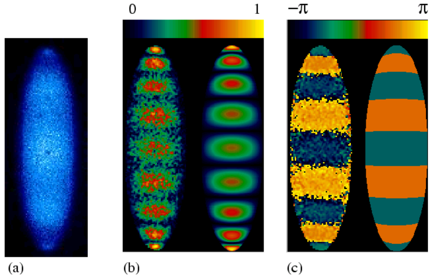
Figure 4. (a) Movie of sideview image data obtained on the plasma of Fig. 3 with \omega_r/2\pi=1.00 MHz while driving a (9,0) mode at \omega_{9,0}/2\pi=2.952 MHz. Comparison of the amplitude (b) and phase (c) extracted from the (9,0) mode in (a) with the predictions of linear theory. The theory predictions are on the right.
