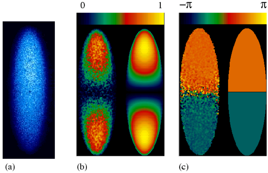
Figure 3. (a) Movie of sideview image data obtained on a plasma with \omega_r/2\pi=1.00 MHz while driving a (2,0) mode at \omega_{2,0}/2\pi=1.656 MHz. The magnetic field and axial laser beam point up. The ion cloud dimensions are 2z_0 = 0.76 mm and 2r_0 = 0.24 mm, and the density n_0 = 2.70 \times 10^9 cm ^{-3} . Comparison of the amplitude (b) and phase (c) extracted from the (2,0) mode in (a) with the predictions of linear theory. The theory predictions are on the right.
