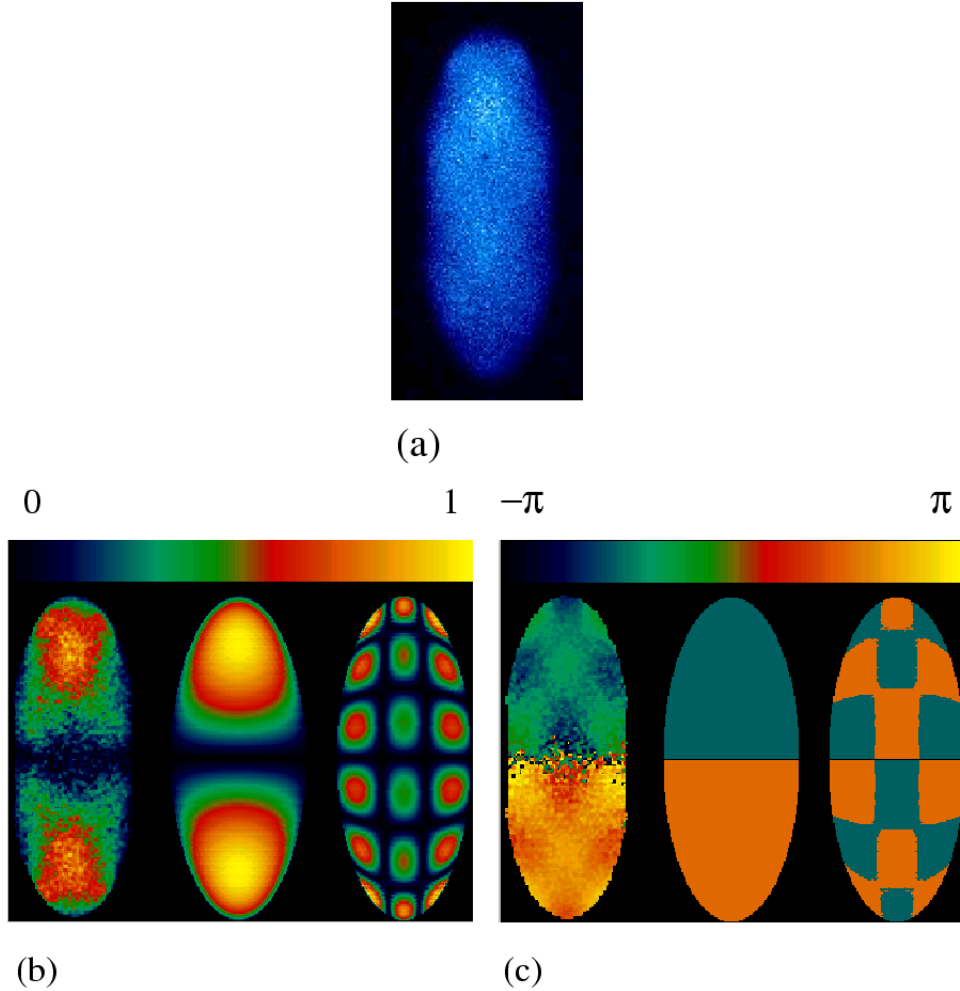
Figure 5. (a) Movie of sideview image data obtained on a plasma with \omega_r/2\pi = 638 kHz while driving with an even drive at 1.619 MHz. At this rotation frequency there is a crossing of the (2,0) mode and an (8,0) mode with a radial node. Comparison of the amplitude (b) and phase (c) extracted from the data in (a) with the predictions of linear theory. The predictions of both the (2,0) and (8,0) modes are given. For this plasma 2z_0 = 0.70 mm and 2r_0 = 0.29 mm.
