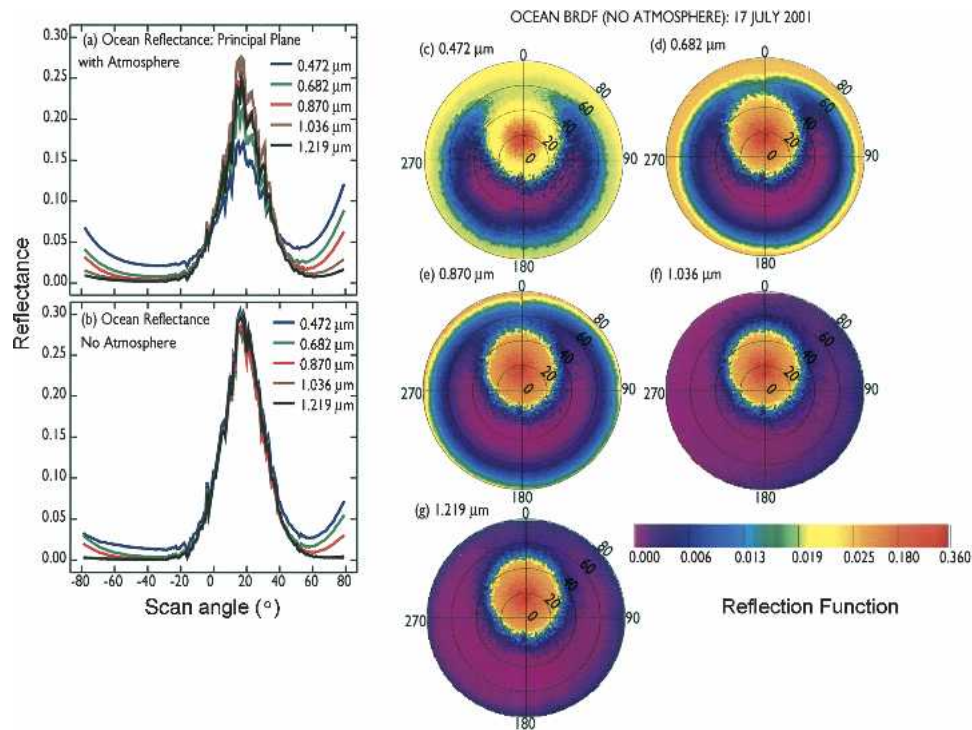
FIG. 6. Illustration of atmospheric correction. (a), (b) The angular distribution of bidirectional reflectance in the principal plane for measurements taken on 17 Jul 2001 at 36.96^{\circ}\text{N} , 75.72^{\circ}\text{W} in the vicinity of Chesapeake Light ( 36.91^{\circ}\text{N} , 75.71^{\circ}\text{W} ) before and after atmospheric correction. (c)–(g) The full atmospherically corrected BRDF for five CAR spectral channels in the visible and near-infrared. The broad reflectance peak represent the sun glint for an average solar zenith angle \theta_0 = 16.23^{\circ} .
