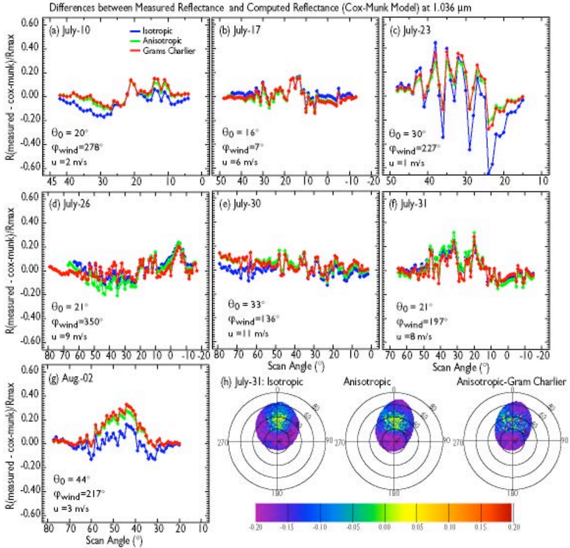
Figure 11. Normalized differences between measurements and computed reflectance using isotropic Cox-Munk, and anisotropic Cox-Munk without and with Gram Charlier expansion (a to g) for the brightest part of the sunglint where computed reflectance R > 0.02 . (h) shows the differences for the entire high glint region for 31 July, to serve as an illustration for the other cases.
