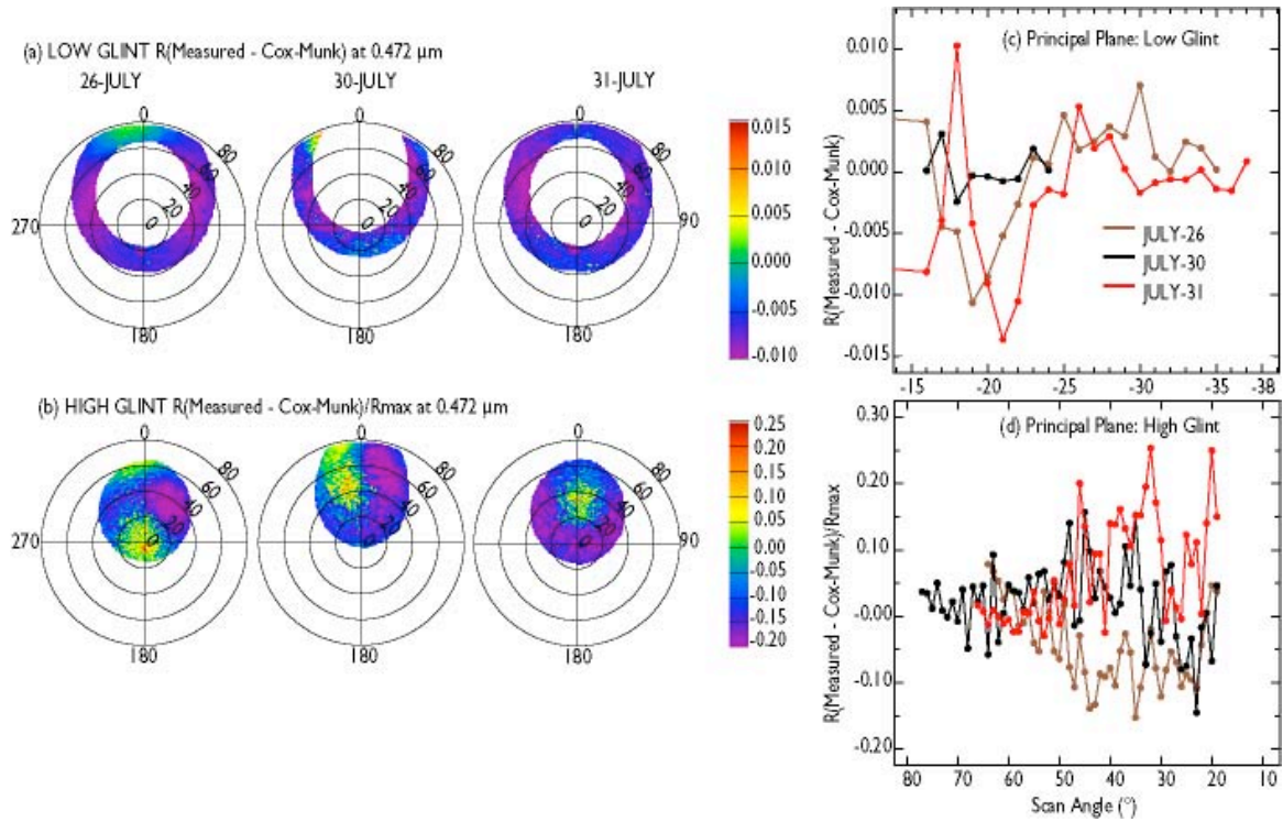
Figure 13. Comparison of differences between measurements and computed reflectance using anisotropic Cox-Munk with Gram Charlier expansion for both high glint and low glint for the three cases with the strongest wind (8-11 ms -1 ).
