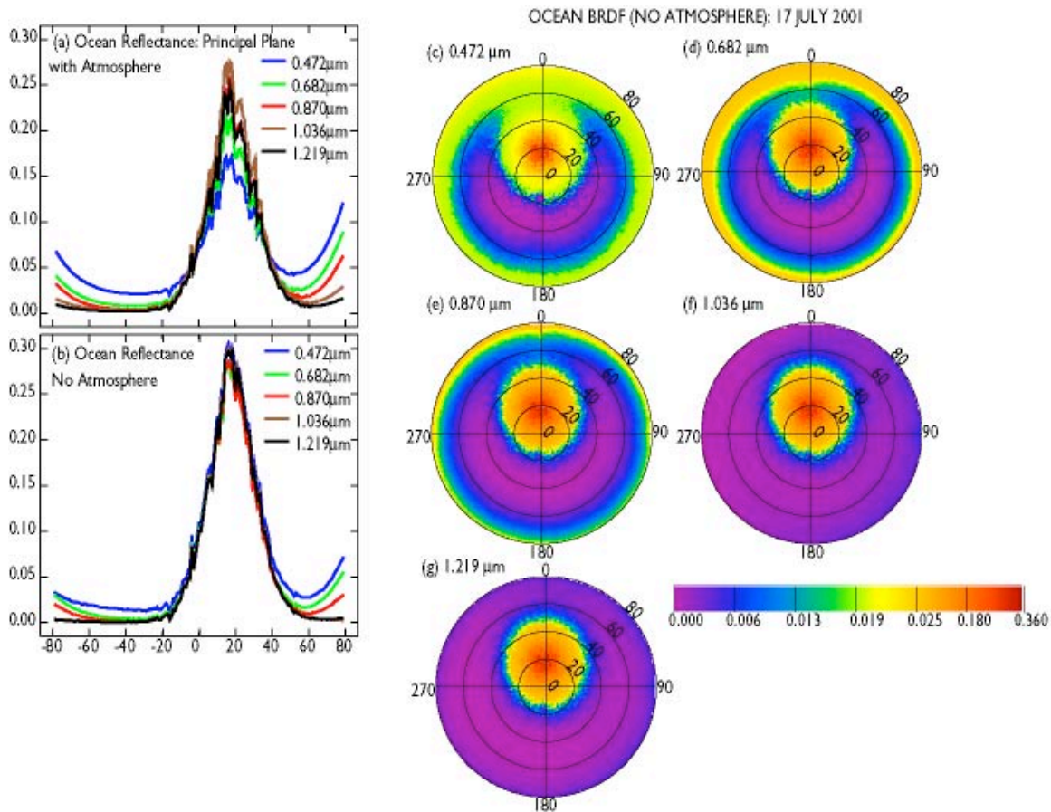
Figure 6. Illustration of atmospheric correction. Panels (a) and (b) show the angular distribution of bidirectional reflectance in the principal plane for measurements taken on 17 July 2001 at (36.96°N, 75.72°W) in the vicinity of Chesapeake Light (36.91°N, 75.71°W) before and after atmospheric correction. Panels (c) through (g) show the full atmospherically corrected BRDF for five CAR spectral channels in the visible and near-infrared. The broad reflectance peak represent the sunglint for an average solar zenith angle \theta_0 = 16.23^\circ .
