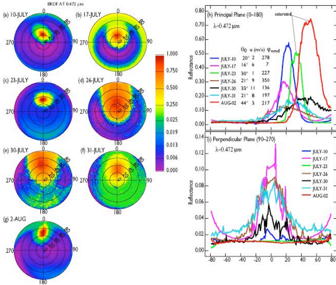
Figure 7. Spectral BRDF at 0.472 \mu\text{m} for seven cloud-free cases obtained by CAR between 10 July and 2 August 2001 during CLAMS. The transects through and perpendicular to the plane of the Sun are also given. The effect of different illumination and wind conditions on the intensity, size, orientation, and location of sunglint are clearly seen.
