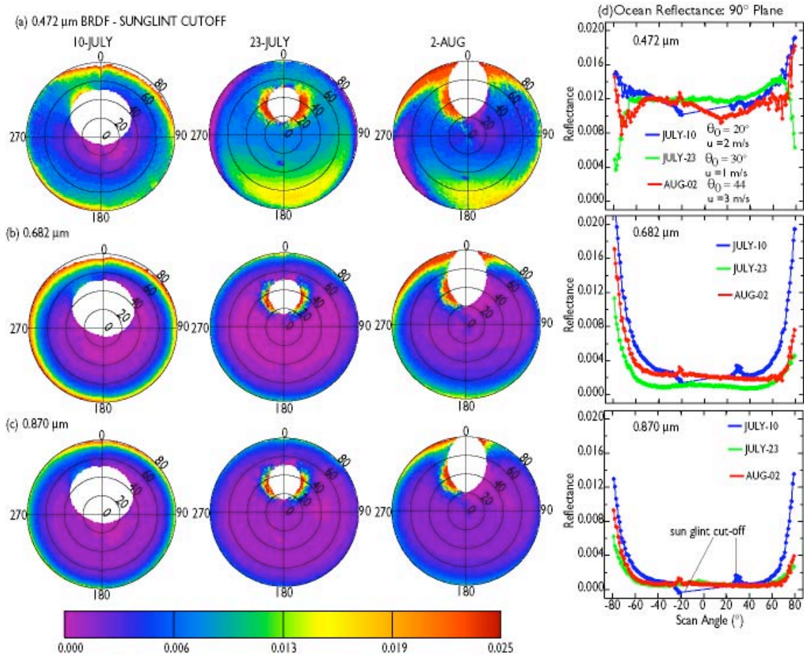
Figure 9. Comparison of spectral BRDF for cases with low wind speeds on 10 and 23 July and 2 August at three CAR channels (0.472, 0.682, and 0.870 \mu\text{m} ) and with the sun glint cutoff to allow more details of the variation of BRDF with view zenith angle.
