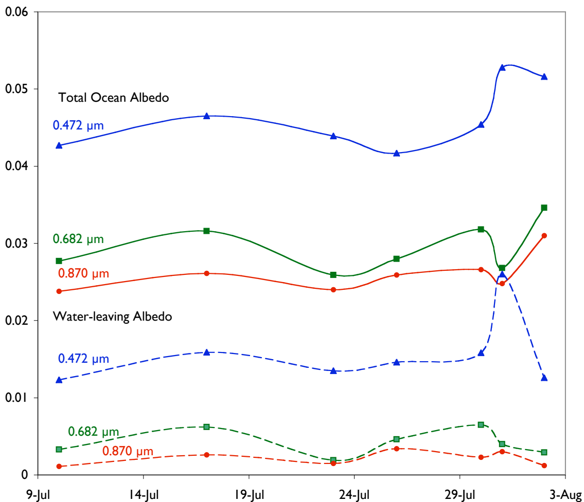
Figure 10. Total Ocean spectral albedo and average water-leaving (total albedo excluding the sunglint) for seven cloud-free cases of CAR measurements over the Atlantic off the U.S. east coast during the CLAMS field experiment campaign from 10 July – 2 August 2001.
