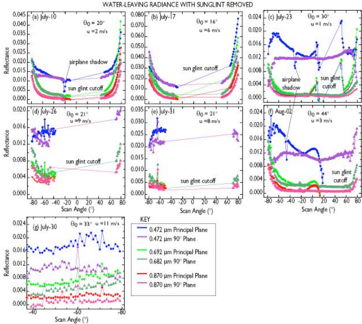
Figure 8. Water-leaving BRDF in the principal and perpendicular plane of the Sun at three CAR channels (0.472, 0.682, and 0.870 \mu\text{m} ) for seven cloud-free cases with various conditions. On average, even though the illumination conditions are different, water-leaving BRDFs do not seem to vary much from case to case. Note that 31 July measurements were obtained in deep Ocean unlike the other cases where measurements were obtained in the proximity of the coastline. The sunglint has been cutoff so as to be able to amplify the low varying BRDFs.
