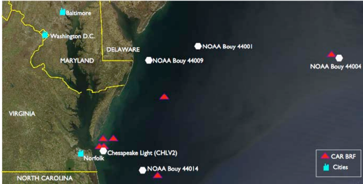
Figure. 1. Locations of airborne measurements of bidirectional reflectance distribution function (BRDF) obtained during the CLAMS field experiment from 10 July- 2 August 2001 using NASA's Cloud Absorption Radiometer (CAR). The background image on which the BRDF locations are mapped is a true color image of Terra Moderate Imaging Spectroradiometer (MODIS) acquired on 13 April of 2003.
