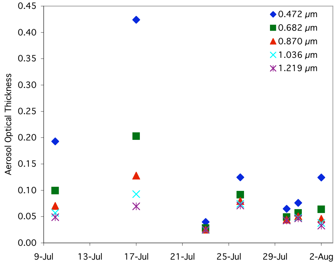
Figure 5. Variation of \tau_a^{\text{aircraft}}(\lambda) as measured by Ames Airborne Tracking Sun-photometer (AATS) during the CLAMS field experiment campaign at the time of BRDF measurements.
