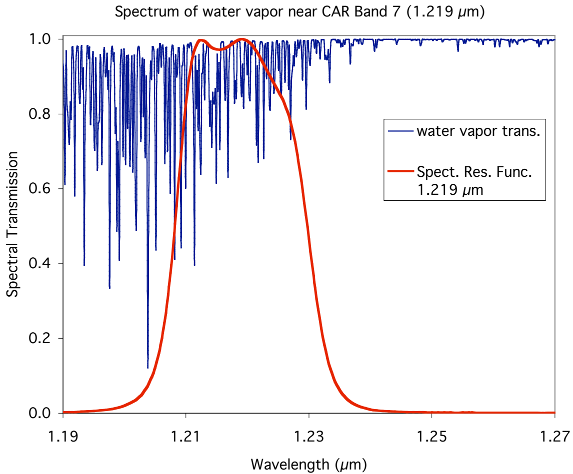
Figure 4. Calculated vertical atmospheric transmission of water vapor averaged over 1 \text{ cm}^{-1} for the CAR band at a wavelength of 1.219 \mu\text{m} for total column water vapor q = 3.15 \text{ g cm}^{-2} ( 2.16 \text{ g cm}^{-2} above the aircraft) on 10 July 2001. The spectral response function at the same wavelength is superimposed.
