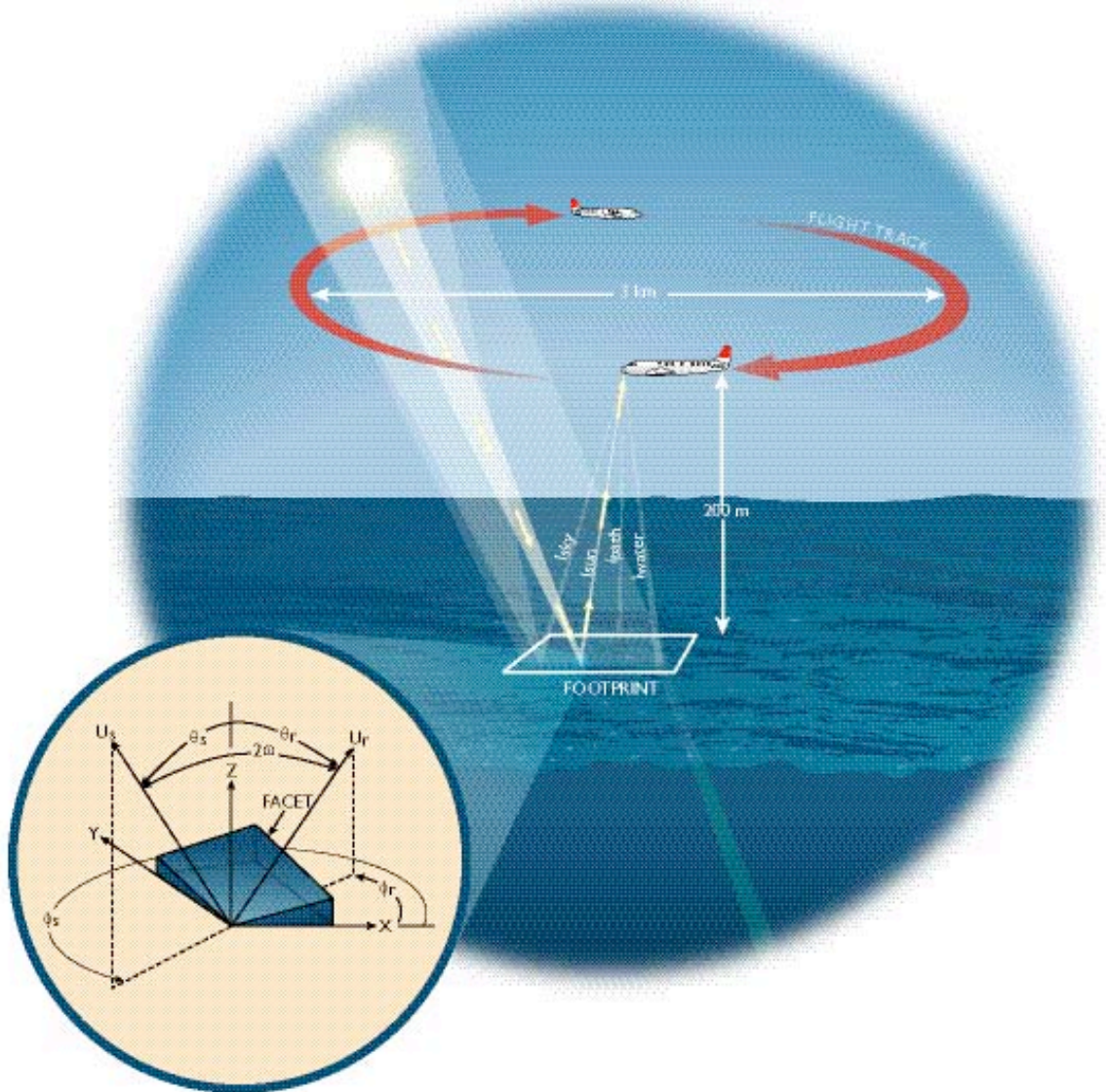
Figure 2. Contributions to instant ocean radiance received by CAR aboard an aircraft scanning the surface from a height H meters above as the aircraft traces a clockwise circular flight track for measuring surface bidirectional reflectance from nadir to the horizon, as well as much of the transmittance from near zenith to the horizon. The inset (modified after Zeiss et al. 1999) shows the geometry of facet reflection with unit vectors U_s and U_r pointing toward the Sun and the sensor, respectively, from the origin of a right-handed coordinate system located at the reflection point.
