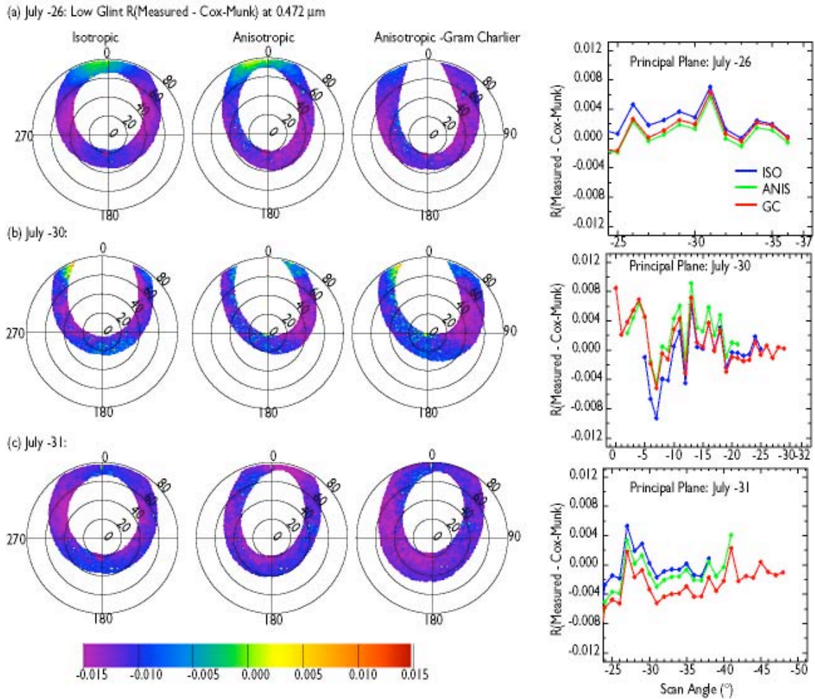
Figure 12. Differences between measurements and computed reflectance using isotropic Cox-Munk, and anisotropic Cox-Munk without and with Gram-Charlier expansion in the darkest part of the sunglint reflectance ( 0.001 < R < 0.02 ).
