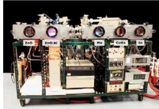
Figure 10. Large area sputtering vacuum systems
