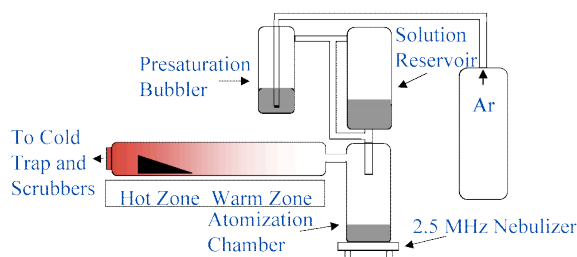
FIGURE 16. Schematic for spray CVD apparatus.
