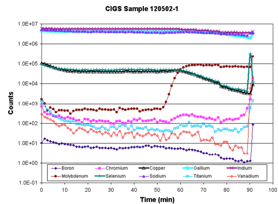
Figure 13. SIMS depth profile for CIGS sample.
