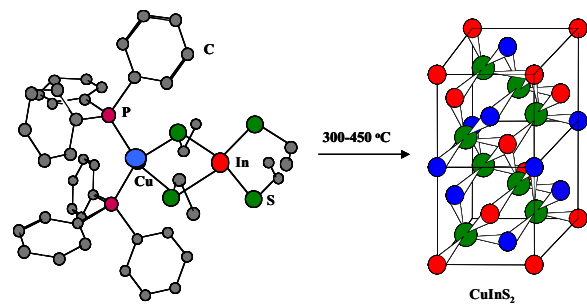
Figure 15. Pyrolysis of SSP [\{PPh_3\}_2Cu(SET)_2-In(SET)_2] , to produce CuInS_2 .
