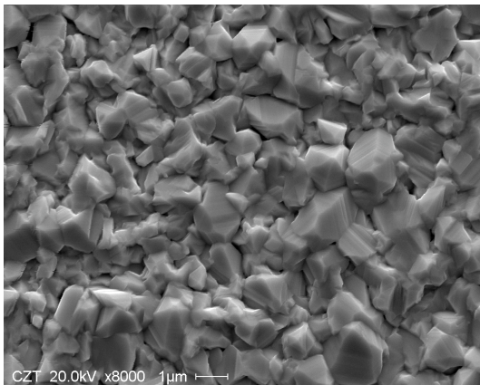
Figure 7. SEM image of a CZT film (17% Zn).
