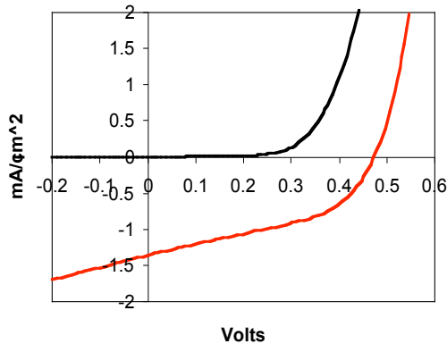
Figure 4. IV curves for Cu/ZnTe/CdSe/TC structures
