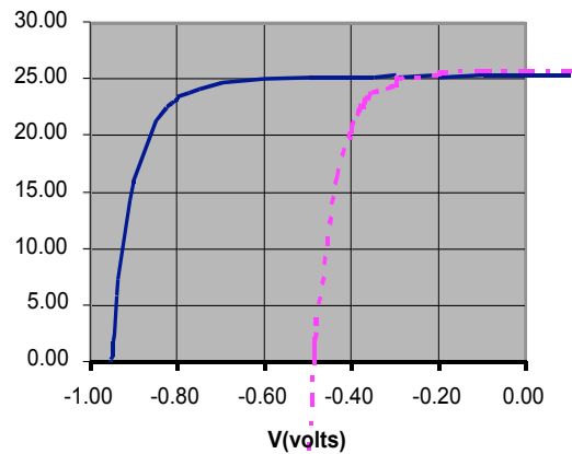
Figure 2. Simulated AM0 IV curves for a tandem device consisting of a 1.55 eV top cell and 0.95 eV bottom CIS cell. Tandem efficiency is 20.1%.
