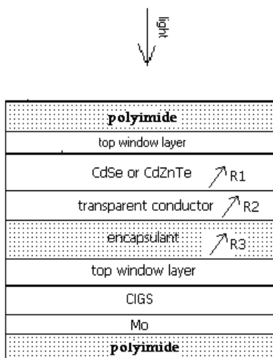
Figure 1. 4-terminal tandem device structure.
