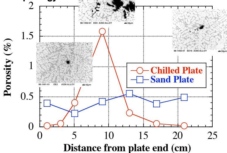
Microporosity distribution and morphology.
