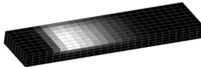
Ratio of shrinkage/gas porosity.
