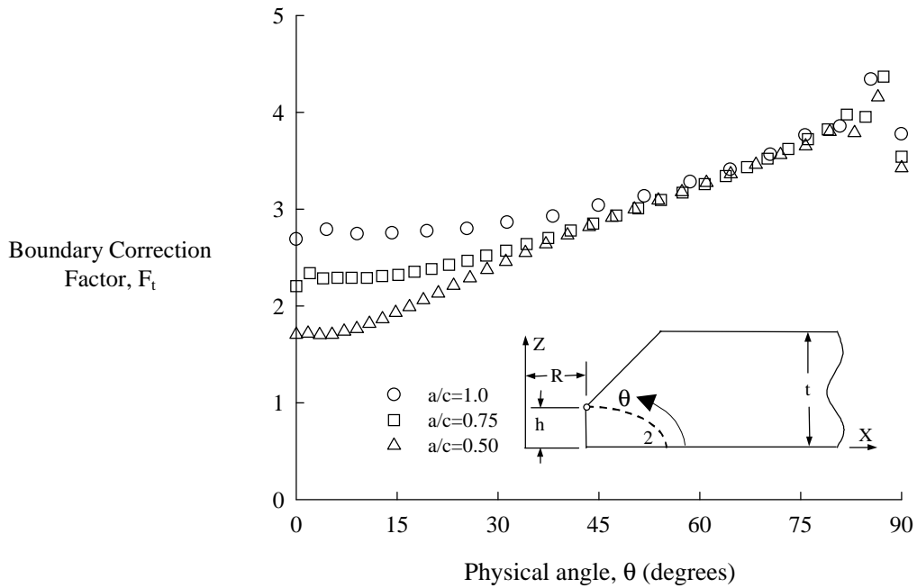
FIGURE 7. BOUNDARY CORRECTION FACTORS, F_t , FOR CRACK LOCATION 2 UNDER TENSION, h/t = 0.25
