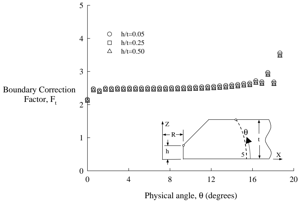
FIGURE 15. BOUNDARY CORRECTION FACTORS, F_t , FOR CRACK LOCATION 5 UNDER TENSION, h/t = 0.05, 0.25, 0.50 ; AND a/c = 1.0
