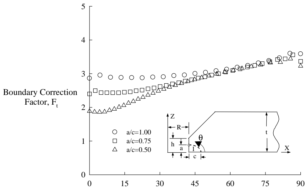
FIGURE 3. BOUNDARY CORRECTION FACTORS, F_t , FOR CRACK LOCATION 1 UNDER TENSION, h/t = 0.05
