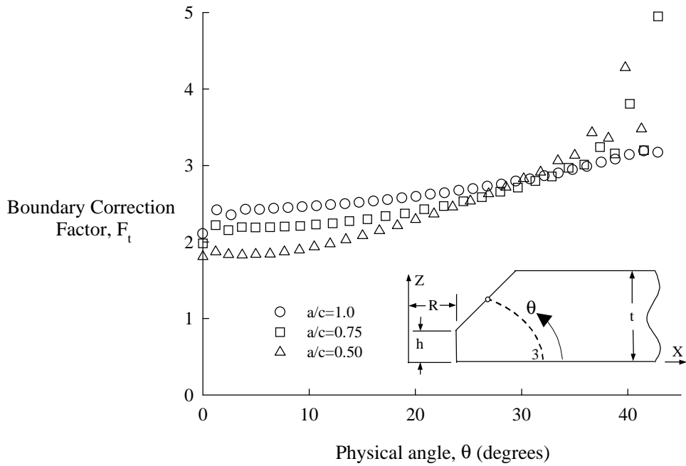
FIGURE 9. BOUNDARY CORRECTION FACTORS, F_t , FOR CRACK LOCATION 3 UNDER TENSION, h/t = 0.05
