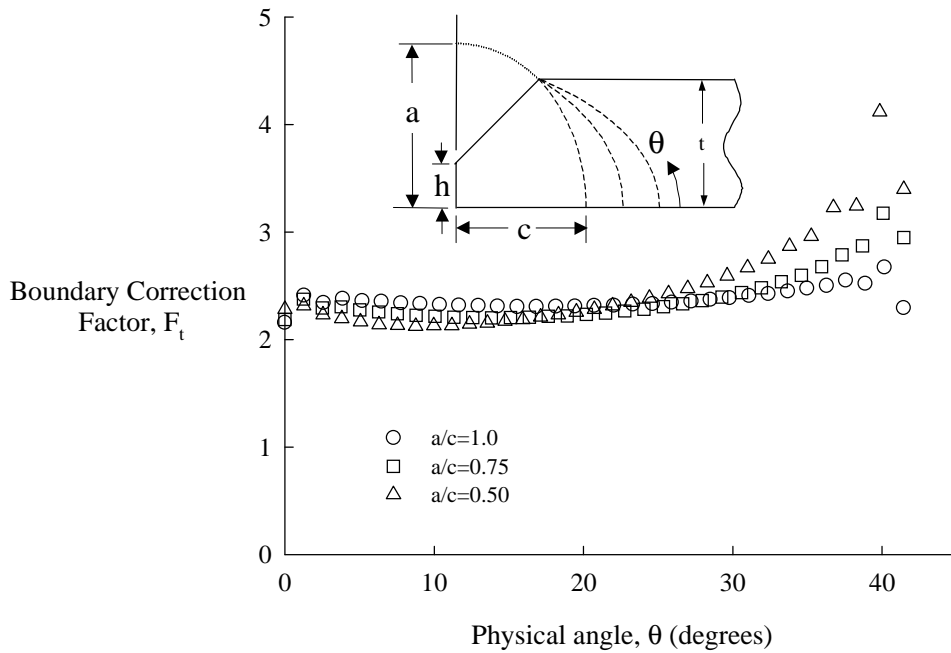
FIGURE 12. BOUNDARY CORRECTION FACTORS, F_t , FOR CRACK LOCATION 4 UNDER TENSION, h/t = 0.05
