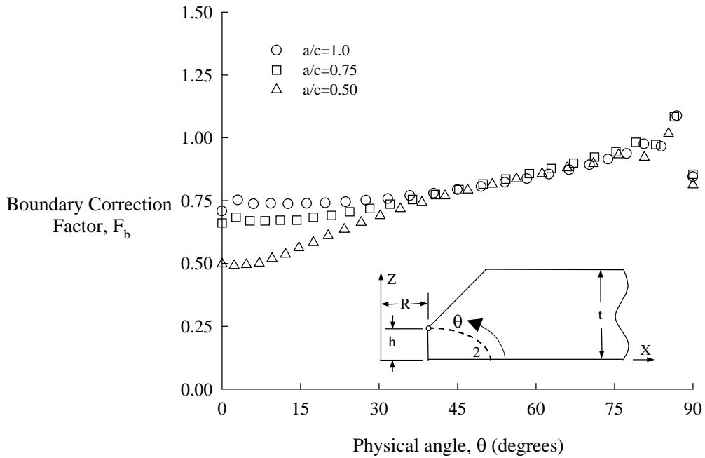
FIGURE 19. BOUNDARY CORRECTION FACTORS, F_b , FOR CRACK LOCATION 2 UNDER BENDING, h/t = 0.05
