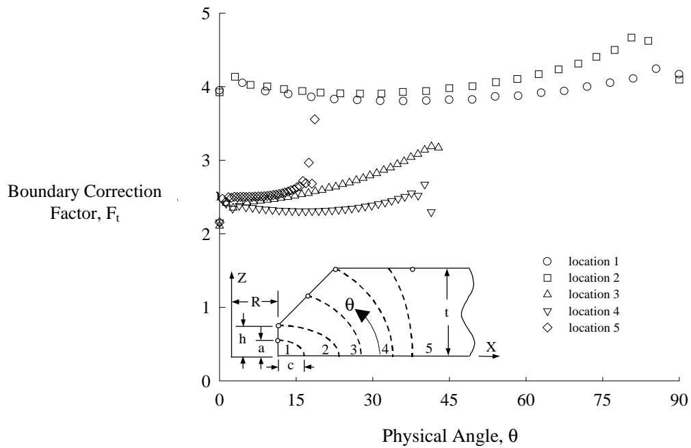
FIGURE 43. EFFECT OF CRACK LOCATION ON BOUNDARY CORRECTION FACTOR FOR h/t = 0.05 ; a/c = 1.0
