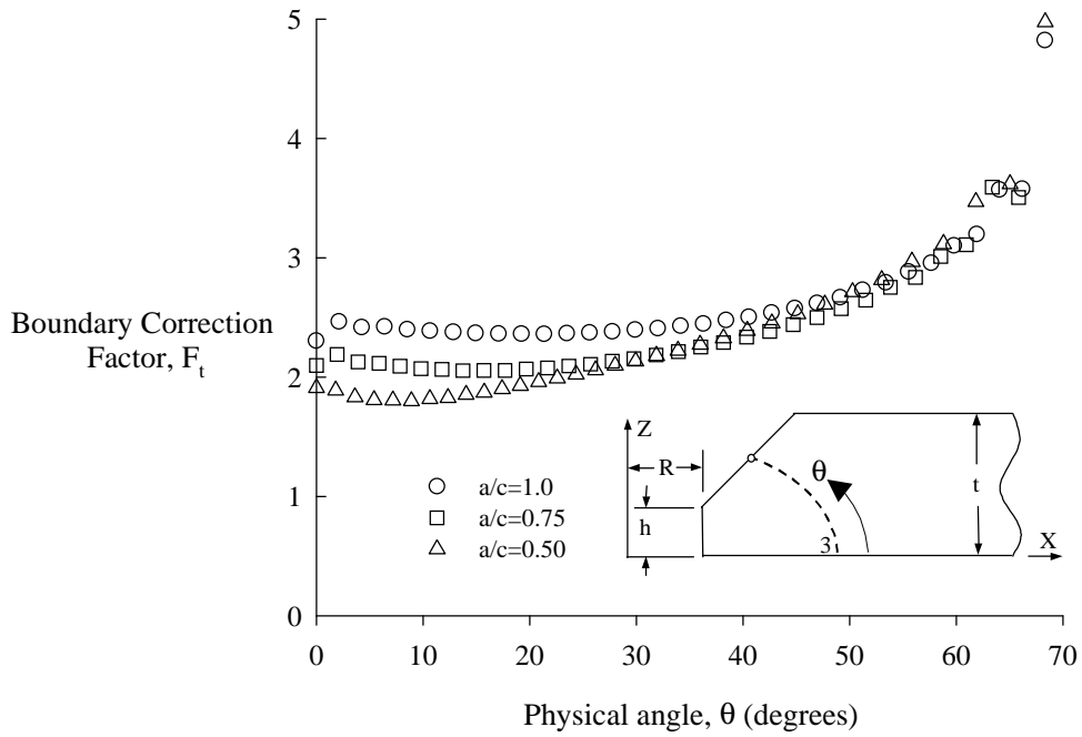
FIGURE 11. BOUNDARY CORRECTION FACTORS, F_t , FOR CRACK LOCATION 3 UNDER TENSION, h/t = 0.50
