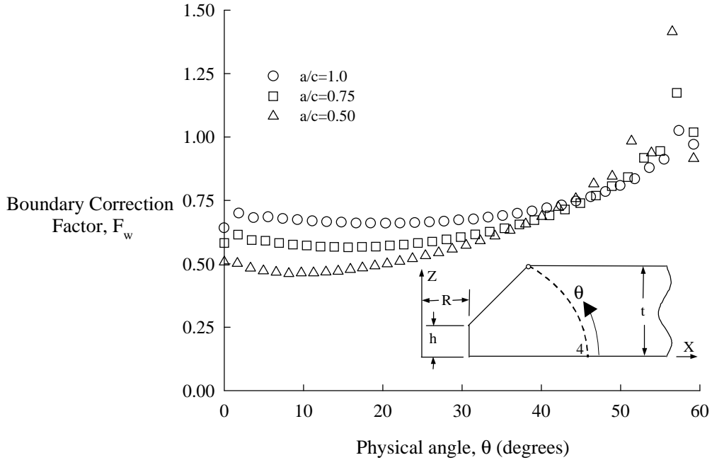
FIGURE 39. BOUNDARY CORRECTION FACTORS, F_w , FOR CRACK LOCATION 4 UNDER WEDGE LOADING, h/t = 0.25
