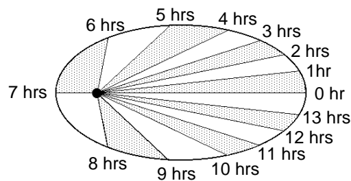
Time Versus Area Swept by an Orbit
