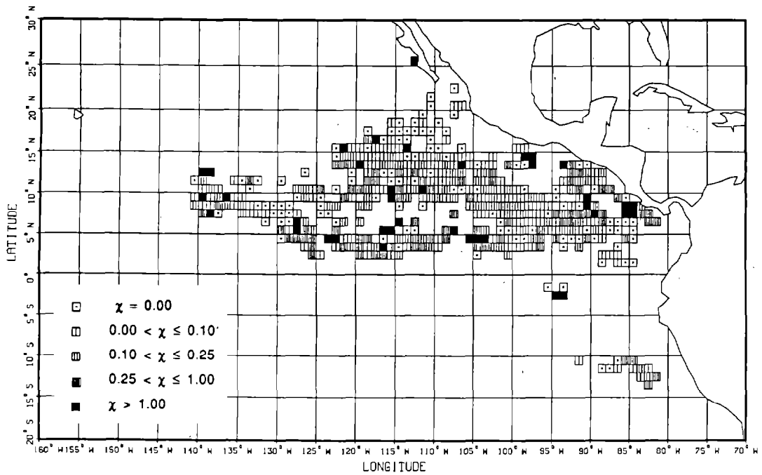
Figure 8 A: The dolphin kill-per-set rates, and B: kill-per-ton rates, by 1^\circ quadrats, for observed U.S. tuna purse seine trips in 1988.
