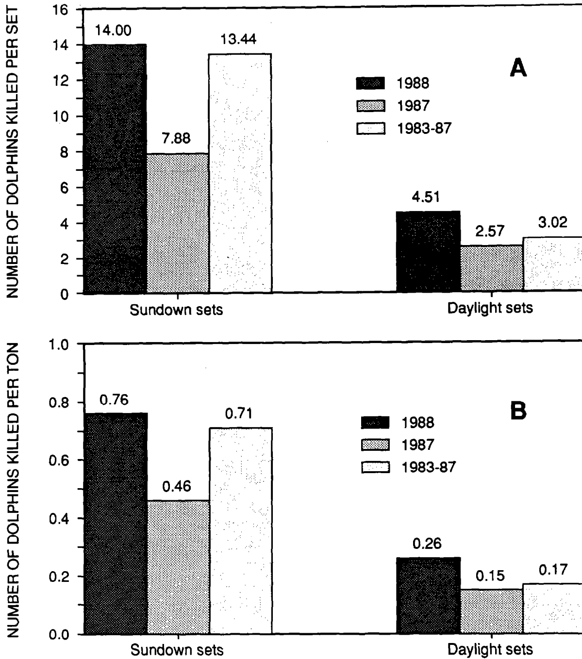
Figure 7 A: The dolphin kill-per-set rates, and B: kill-per-ton rates, by sundown sets versus daylight sets, for observed U.S. tuna purse seine trips in the eastern tropical Pacific Ocean in 1988, 1987 and the 1983-87 average.
