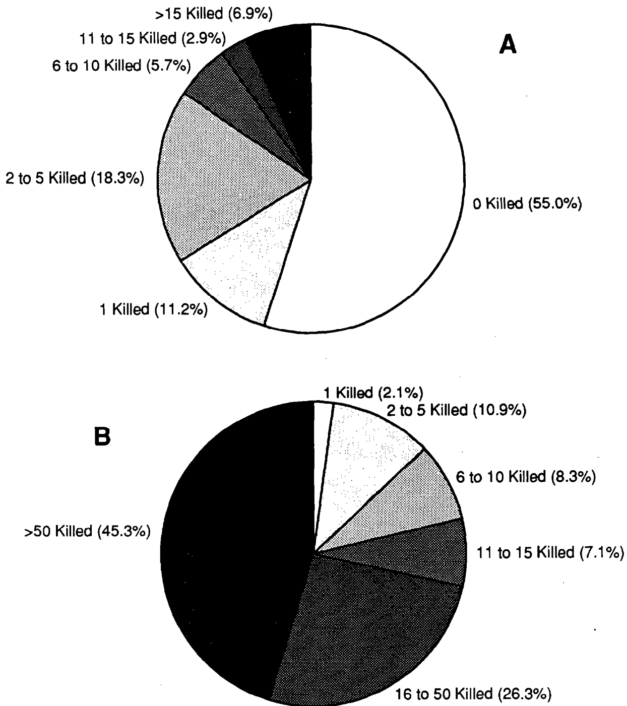
Figure 5 A: The proportion of all dolphin sets that resulted in dolphin mortalities of 0, 1, 2-5, 6-10, 11-15 and more than 15; and B: the proportion of the total dolphin mortality that resulted from sets with dolphin mortalities of 1, 2-5, 6-10, 11-15, 16-50 and more than 50, for observed U.S. tuna purse seine trips in the eastern tropical Pacific Ocean in 1988.
