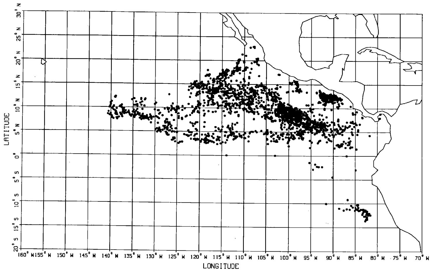
Figure 9A. Locations of offshore spotted dolphin sightings reported by observers aboard U.S. tuna purse seiners in 1988.
