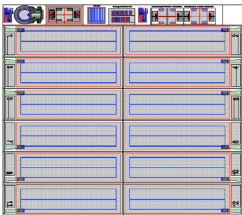
Figure 19: Photolithography mask for cat's eye focal plane array
