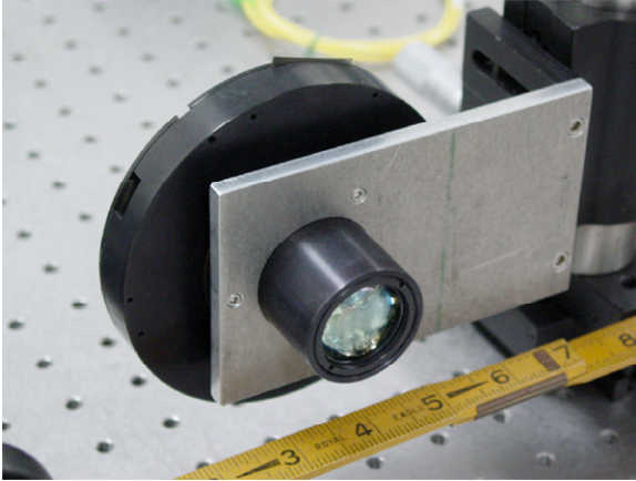
Figure 18: the diffraction limited cat's eye modulating retro-reflector
