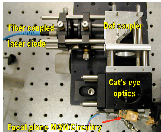
Figure 12: A cat's eye modulating retroreflector node
