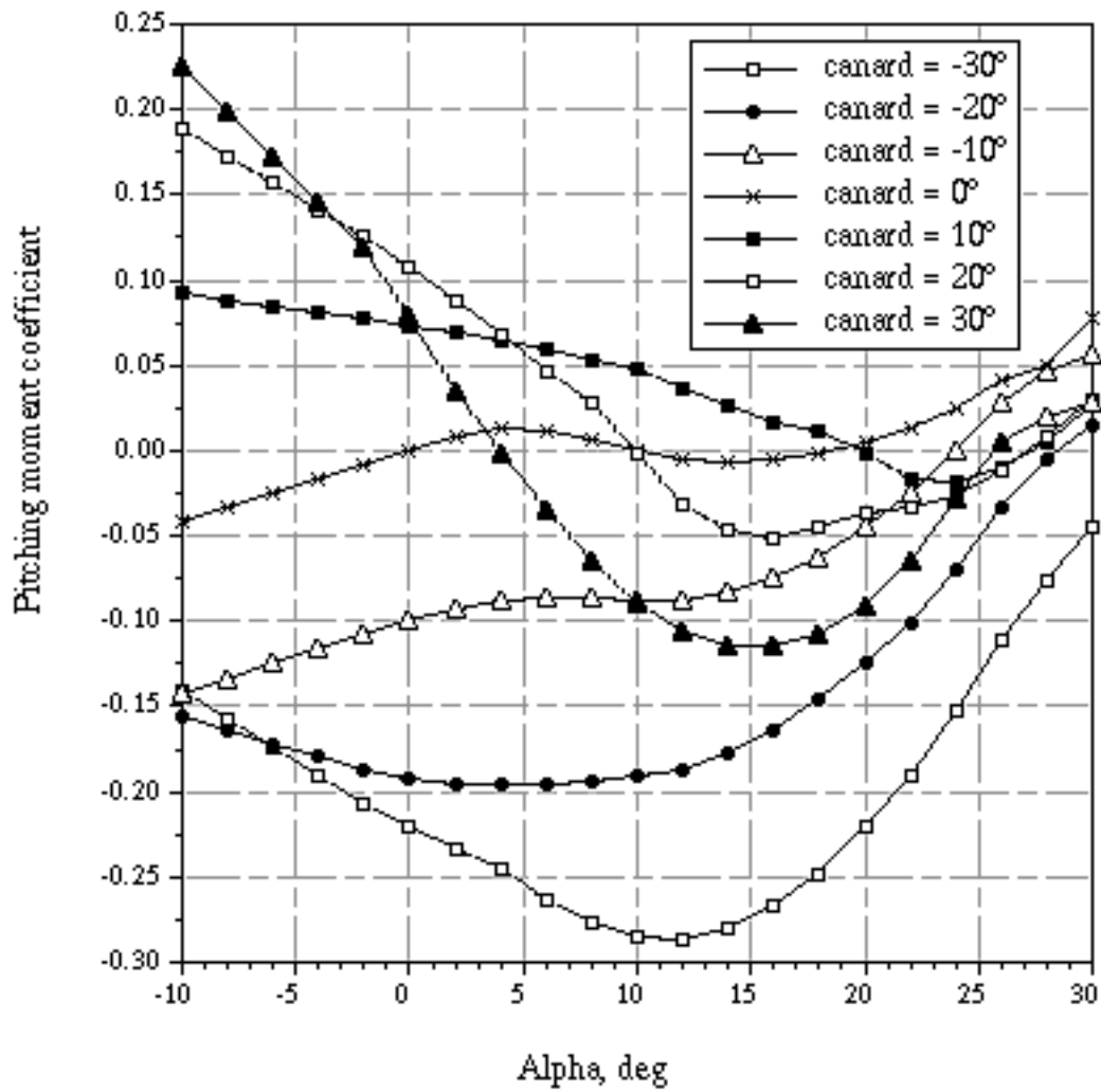
Figure 24. Pitching moment coefficient for various canard deflections, M = 0.2
