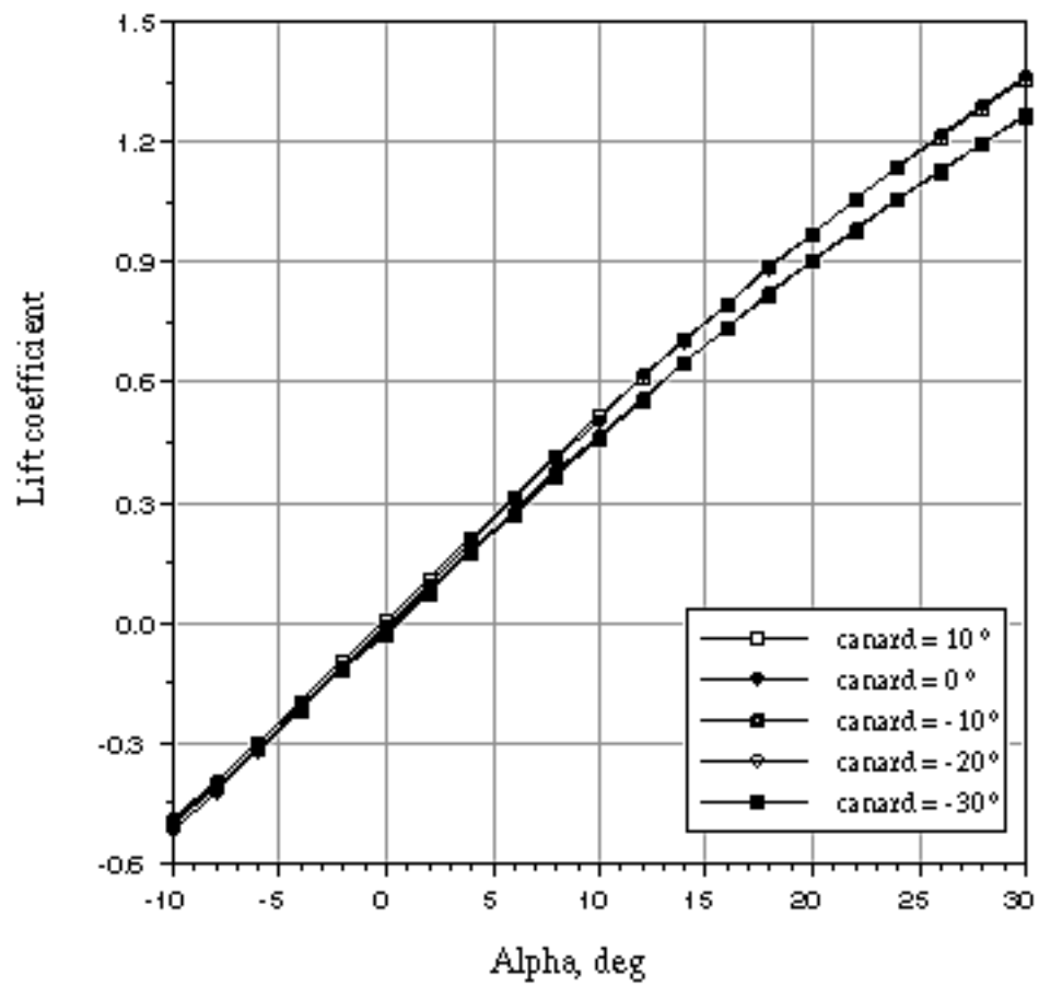
Figure 4. Lift coefficient for various canard deflections, M = 0.2
