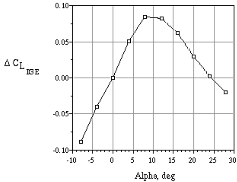
Figure 6. Lift coefficient increment due to ground plane influence
