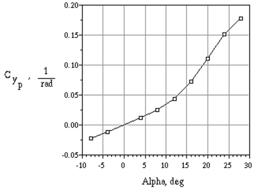
Figure 40. Side force coefficient due to roll rate
