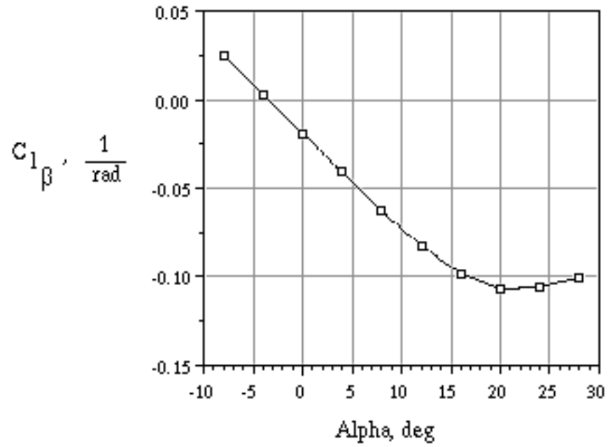
Figure 42. Rolling moment coefficient due to sideslip
