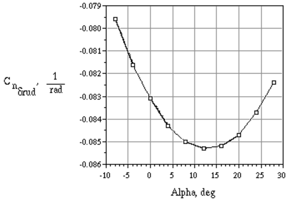
Figure 58. Yawing moment coefficient due to rudder deflection
