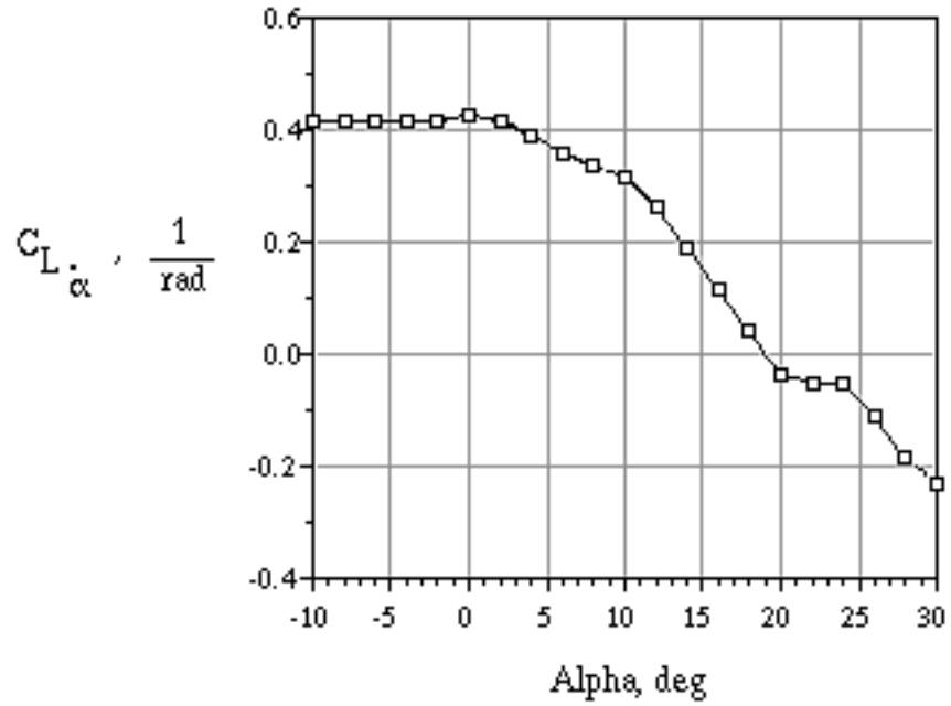
Figure 5. Lift coefficient due to angle-of-attack rate
