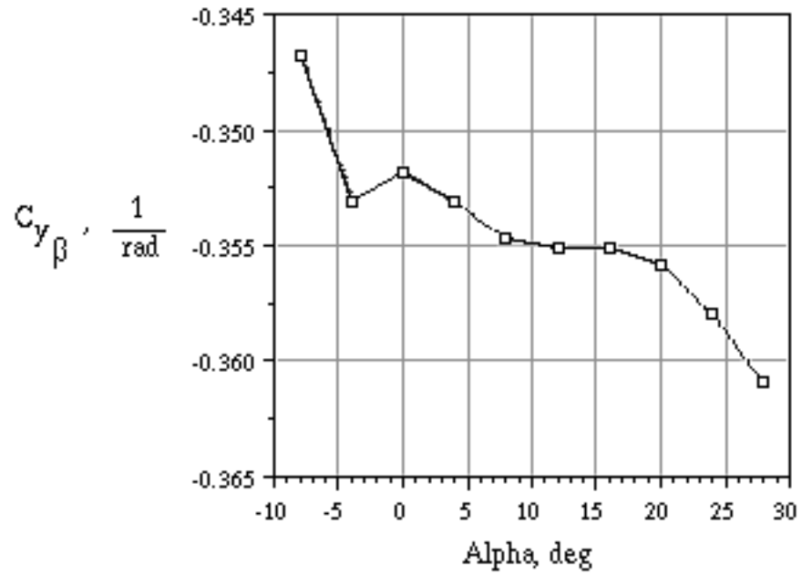
Figure 39. Side force coefficient due to sideslip
