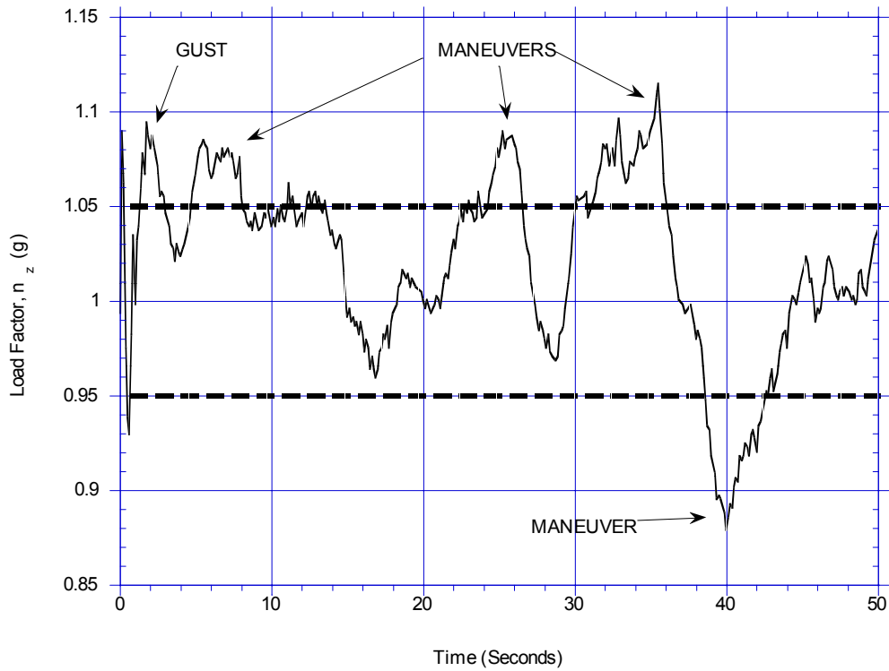
FIGURE 1. APPLICATION OF 2-SECOND RULE FOR MANEUVER-GUST SEPARATION
