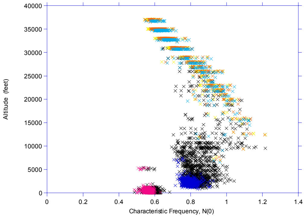
FIGURE 3. ALTITUDE VS CHARACTERISTIC FREQUENCY, N(0)
