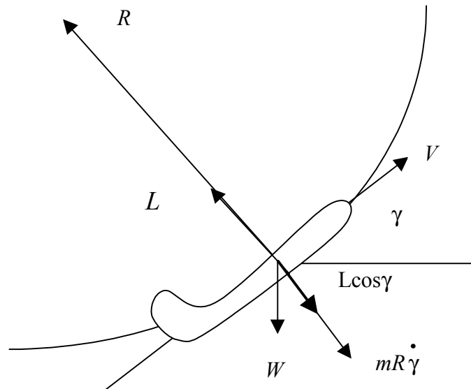
FIGURE A-4. FORCES ON AIRPLANE DURING STEADY SYMMETRICAL PULL-UP
