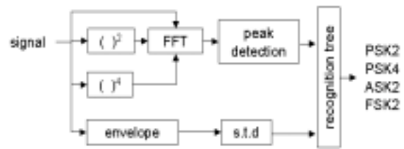
Figure 17. Power-Law Modulation Classifier
