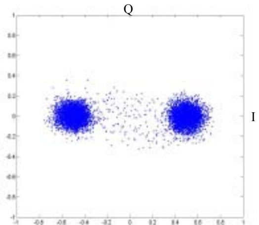
Figure 4 Constellation Diagram of BPSK
