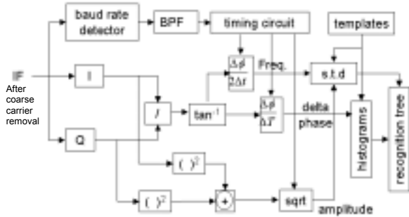
Figure 10. Universal Demodulator
