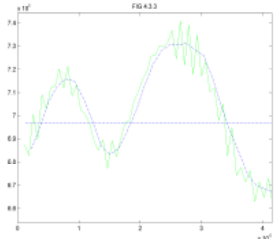
Figure 16 Zero-crossing Frequency Plot of A FSK Signal
