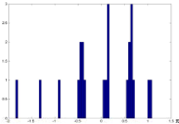
Figure 12 Histogram of Delta-Phase Symbols of DQPSK
