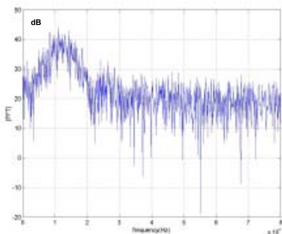
Figure 18 Frequency Spectrum of A QPSK Signal
