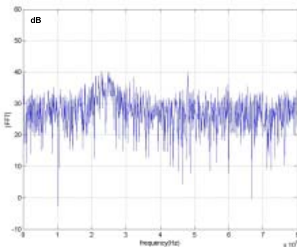
Figure 19 Spectrum of A QPSK Signal with Forth-Power
