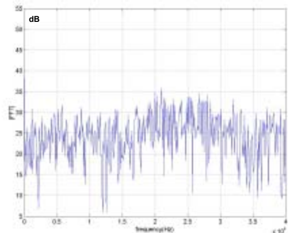
Figure 20 Under-Sampled QPSK Signal with Forth-Power
