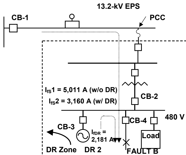
Figure 17. Effects of infeed on system fault current
