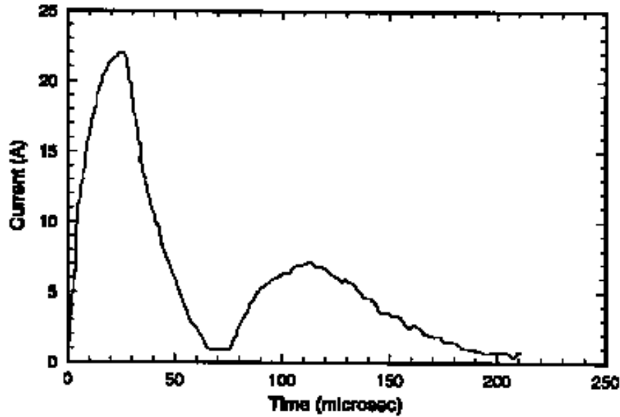
Figure 3: Plot of the current pulse displayed on the FAX.
