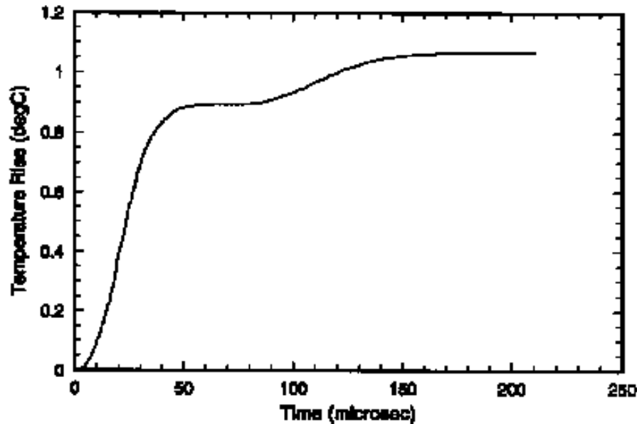
Figure 4: The temperature rise of an FM08 fuse rated at 7 A, under the current pulse given above, when the ambient temperature is in the range 20° C to 25° C.
