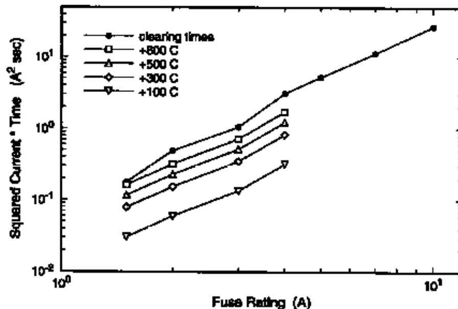
Figure 2: Plot of the i^2 \cdot t values producing various temperature rises in FM08 filaments, as per Ref. (b). Also shown are the i_{int} \cdot t_{int} values from Mr. O'Shea's data.
