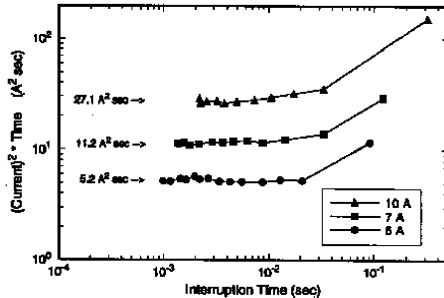
Figure 1: Plot of some of the data obtained by Mr. Peter O'Shea, then of Paramax at GSFC. This data is consistent with the manufacture's curves.
