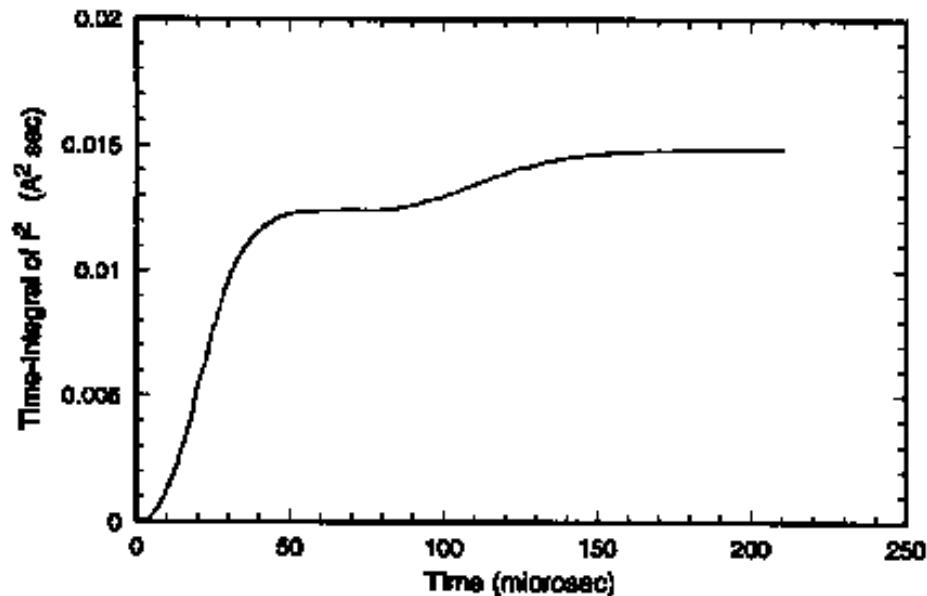
Figure 5: The value of \int_0^t i^2 dt for the subject pulse.
