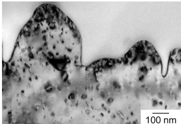
Fig. 6—Bright-field TEM image from a longitudinal cross section of a region of the line showing severe topography after 1.39 \times 10^5 thermal cycles. Numerous prismatic dislocation loops are seen in this grain; however, there is negligible residual dislocation content in the form of segments. The image was taken approximately 6 months after testing, during which time loops grew from an initial average of approximately 4.5 nm to greater than 10 nm due to vacancy coalescence at room temperature. The bottom edge of the micrograph is coincident with the film/substrate interface.
