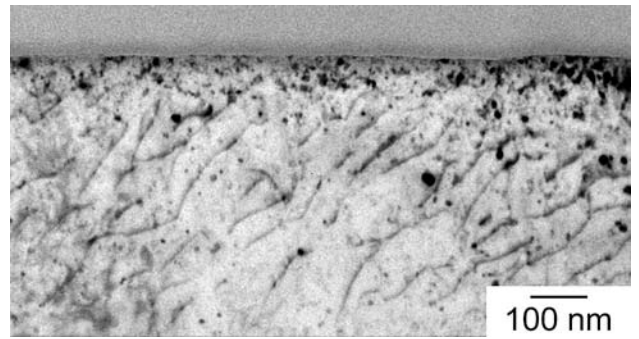
Fig. 7—Bright-field TEM image from a longitudinal cross section of a region of the line showing little topography after 1.39 \times 10^5 thermal cycles. Numerous dislocation segments are visible in this grain. The bottom edge of the micrograph is coincident with the film/substrate interface.
