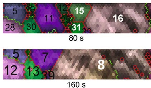
Fig. 8—Example of pairwise comparison of EBSD image quality parameters for growing grains. After the 80 s time increment, grain 16 grew, consuming grains 15 and 31 (among others). It became grain 8 at the 160-s time increment. The lines between grains indicate grain boundaries, with red corresponding to high-angle and green corresponding to low-angle boundaries. Boundaries surrounding single pixels are locations where the diffraction pattern could not be indexed.
