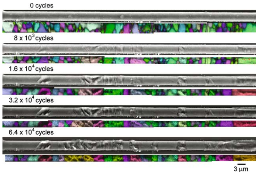
Fig. 1—SEM/orientation map pairs from the same region of the line, showing development of damage in the form of surface topography and grain growth/reorientation after 0, 40, 80, 160, and 320 s of accumulated cycling. Colors represent crystal directions lying parallel to line direction, with the legend given in Fig. 2. This 100\ \mu\text{m} \times 3\ \mu\text{m} region was used for all quantitative grain measurements.
