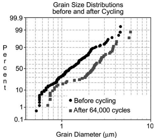
Fig. 3—Grain size distributions from the 100 \mu\text{m} \times 3 \mu\text{m} region of the line, before and after 6.4 \times 10^4 thermal cycles at 200 Hz. The mean (expected value) grain diameter \pm measurement uncertainty increased from 1.4 \pm 0.4 \mu\text{m} to 2.4 \pm 0.4 \mu\text{m} after 320 s of cycling.
