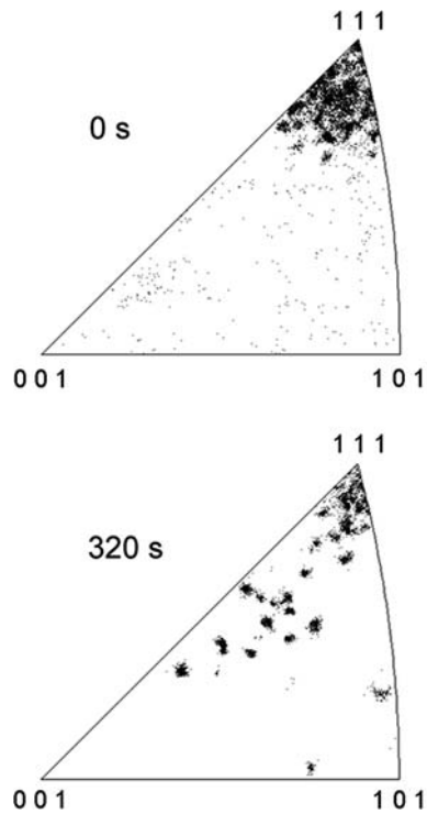
Fig. 5—Inverse pole figures showing surface normal orientations for grains prior to testing (top) and deformed grains after 1.39 \times 10^5 thermal cycles (bottom), as determined by EBSD. Prior to cycling, the specimen showed a \langle 111 \rangle fiber texture, typical of physical-vapor-deposited metals. After cycling, some grains rotated by more than 40 deg.
