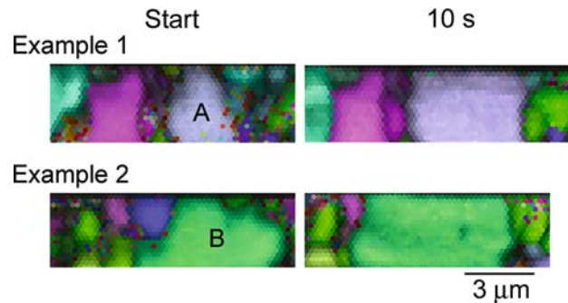
Fig. 4—EBSD maps showing two examples of grain growth that took place after 10 s of testing (2000 thermal cycles). Grain “A” shows an area increase of 114 pct, and equivalent diameter increase from 3.0 \mu\text{m} to 4.4 \mu\text{m} . Grain “B” shows an area increase of 60 pct, and equivalent diameter increase from 4.0 \mu\text{m} to 5.2 \mu\text{m} . Colors represent directions lying parallel to the line direction, with the legend given in Fig. 2.
