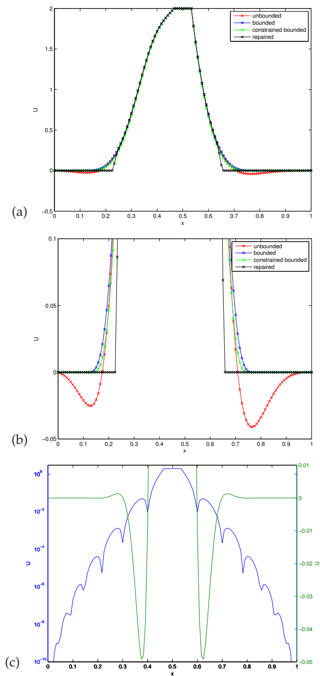
Figure 8: Problem with non-smooth anisotropic solution with the anisotropy ratio 1/k=1/1000 on the mesh with 120 edges on unit boundary: (a) full view and (b) view zoomed, scaled in y direction of 1D cuts along the line y=7/15 , comparison of unbounded, bounded, constrained-bounded and repaired solution; (c) 1D cut of unbounded solution U^u along the diagonal y=1-x , green is U^u with the right linear axis and blue is |U^u| with the left logarithmic axis.
