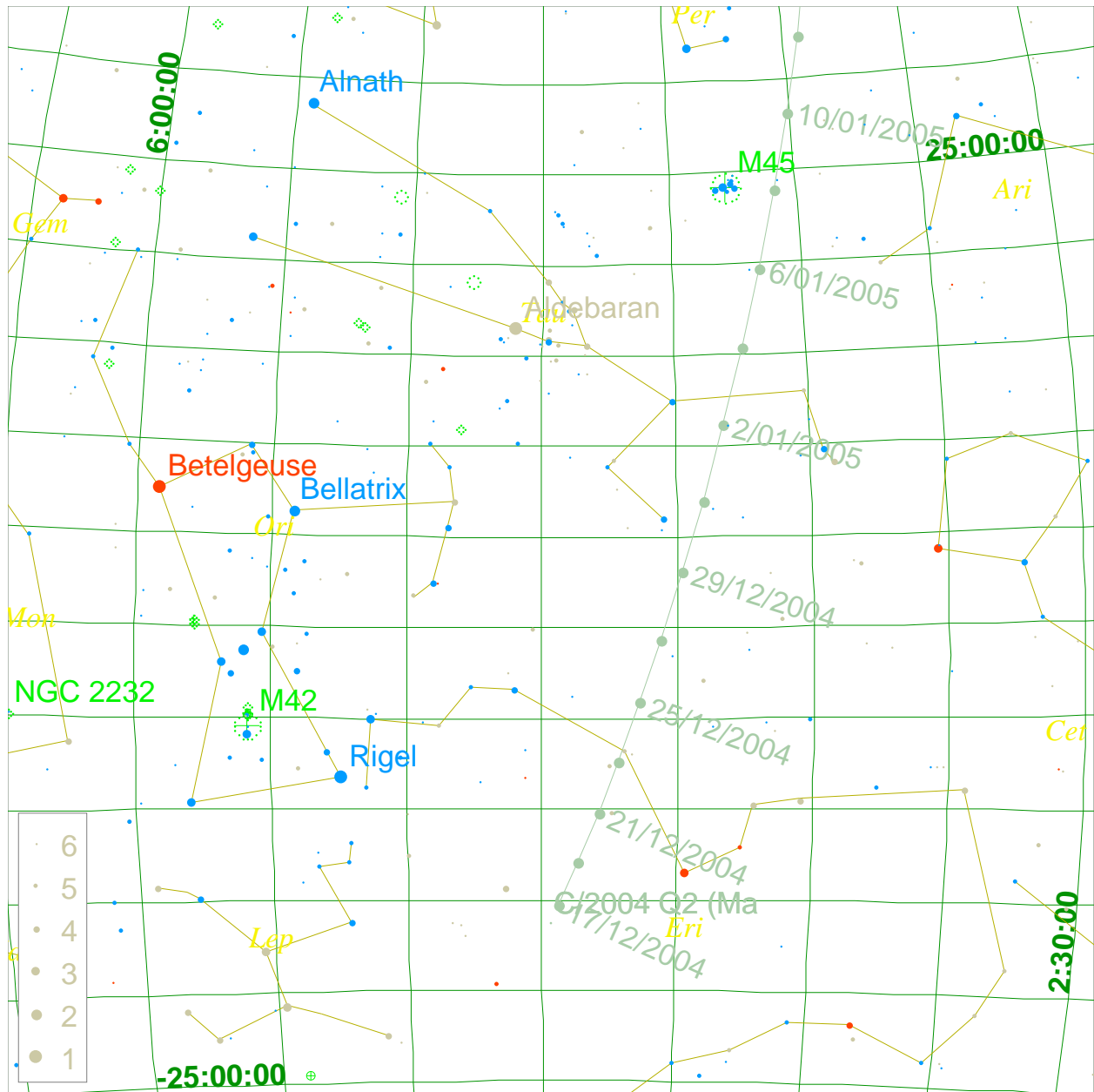
XEphem Geocentric Mean RA/Dec Sky View -- Trail Times are in UTC Cleveland, Ohio
