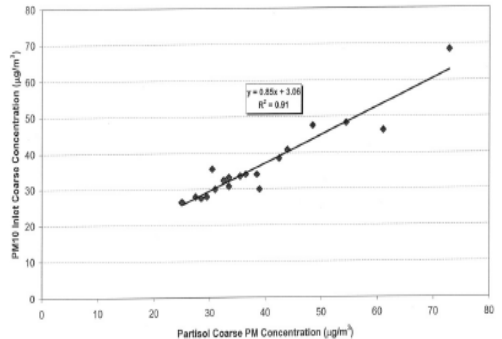
Figure 5. Coarse PM concentrations determined by the 50 L/min \text{PM}_{10} inlet and the R&P Partisol.
