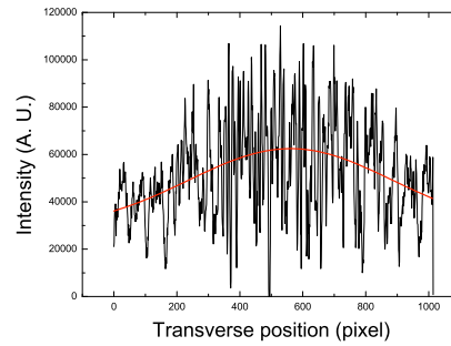
Figure 5: Transverse LIF intensity profile extracted from the 2D CCD image. The red curve is a Gaussian fit to the measured signals.
