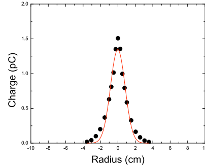
Figure 3: Radial profiles of the trapped barium ions in the PTSX device. The red curve is a Gaussian fit to the measured signals.
