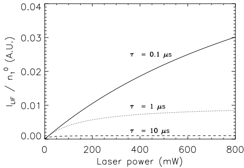
Figure 4: Dependence of LIF intensity I_{LIF} on laser power and characteristic ion transit time \tau .
