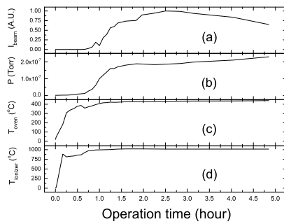
Figure 2: Time evolution of: (a) the beam current generated by the barium ion source; (b) pressure; and (c) and (d) temperatures of the oven and the ionizer.
