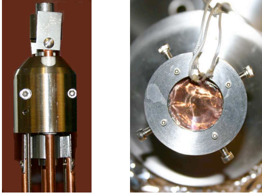
Figure 1: Assembly of tantalum oven tube, platinum mesh ionizer, tungsten heaters, and copper rods (left). Assembly of Pierce electrode, acceleration grid, and deceleration grid on top of the aluminum can (right).
